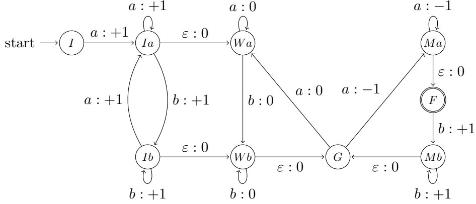
Figure 1: The automaton \mathcal{A}
