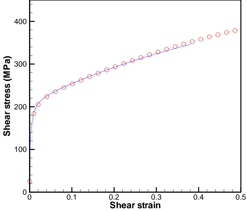
Figure 7: Shear test results : 0° sample (—) and 45° responses (o).
