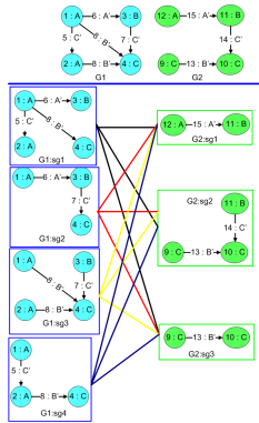
Figure 8: Subgraph matching : A bipartite graph
