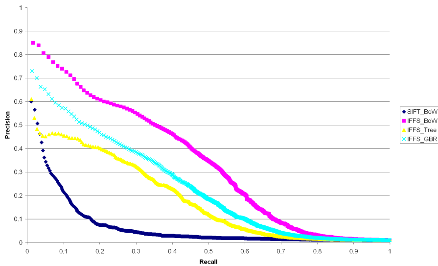
(a) Results on Coil100 database
