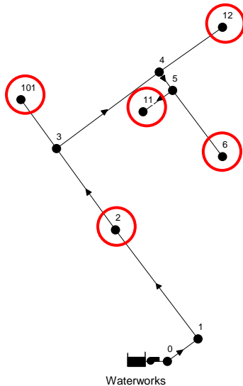
Figure 10 Sketch of the EPANET water network model of the construction area in Farum The red circles indicate the locations that were considered relevant to give an overview of the pollution level. At these locations, the detailed migrant concentration is analysed.
