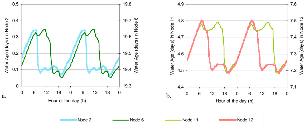
Figure 12 Computation of the water age in the Farum network Due to big differences in age between the different locations, each curve has its own Y-axis, otherwise it would not be possible to see the variations along the day.
