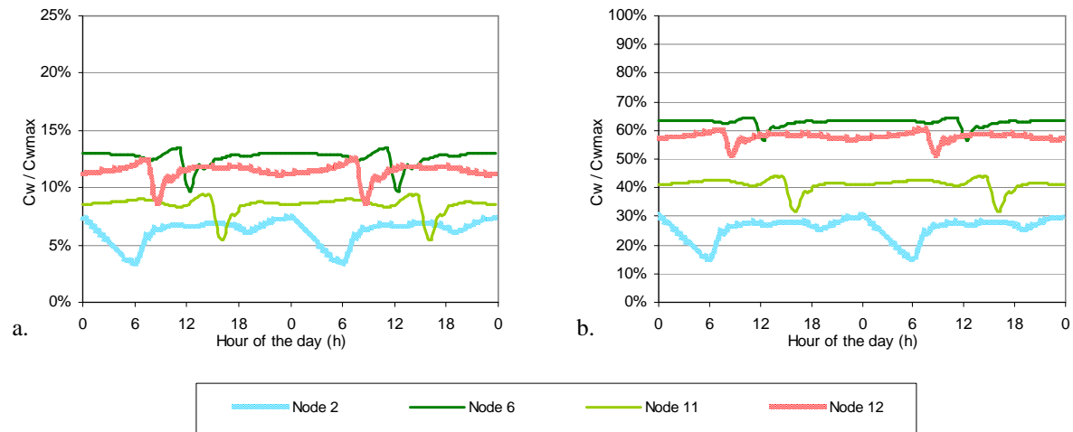
Figure 14 Simulation results for the Farum network: daily variations of the migrant concentration. The two graphs represent the saturation level of species along the day at relevant nodes of the network, for migrant's diffusion coefficient in the water of 10^{-10} m 2 /s for Graph a and 10^{-9} m 2 /s for Graph b. If one considers antioxidants such as Irganox 1010 or Irgafos 168 then the concentration of species in the PE matrix is about 2 g/kg and their partition coefficient at the interface around 1.55 \cdot 10^{-4} , leading to a saturation concentration of 310 \mu g/L.
