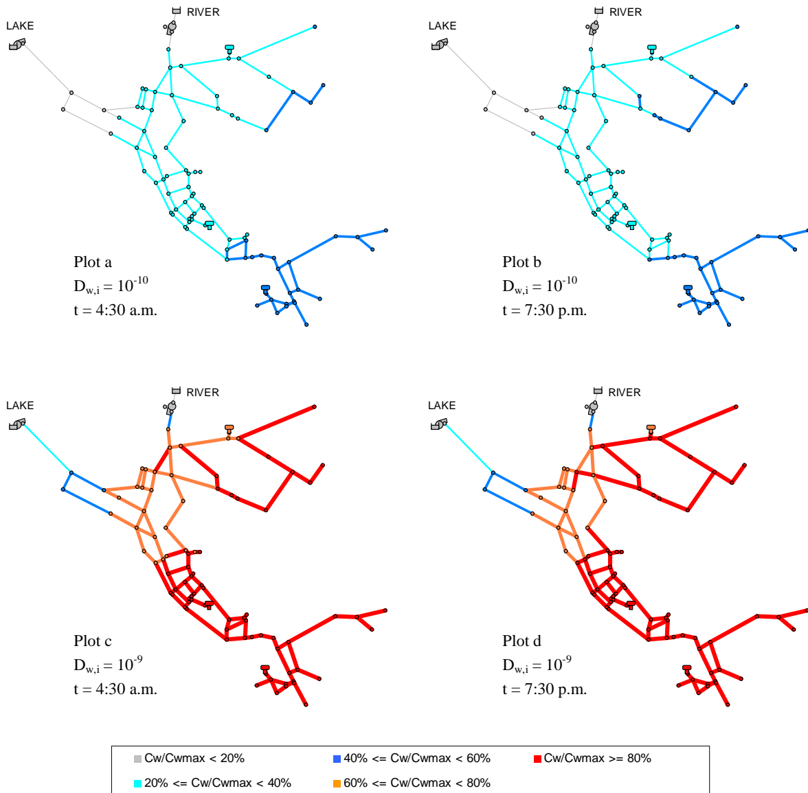
Figure 35 Simulation results for “Net 3”: map-plot of the migrant concentration The figure represents the migrant saturation level in the network when no degradation is simulated at two times of the day. Plots a and b correspond to the case where a diffusion coefficient of the migrants in the water is 10^{-10} \text{ m}^2/\text{s} , and plots c and d to the case where it is 10^{-9} \text{ m}^2/\text{s} . If one considers antioxidants such as Irganox 1010 or Irgafos 168 then the concentration of species in the PE matrix is about 2 g/kg and their partition coefficient at the interface around 1.55 \cdot 10^{-4} , leading to a saturation concentration of 310 \mu\text{g}/\text{L} .
