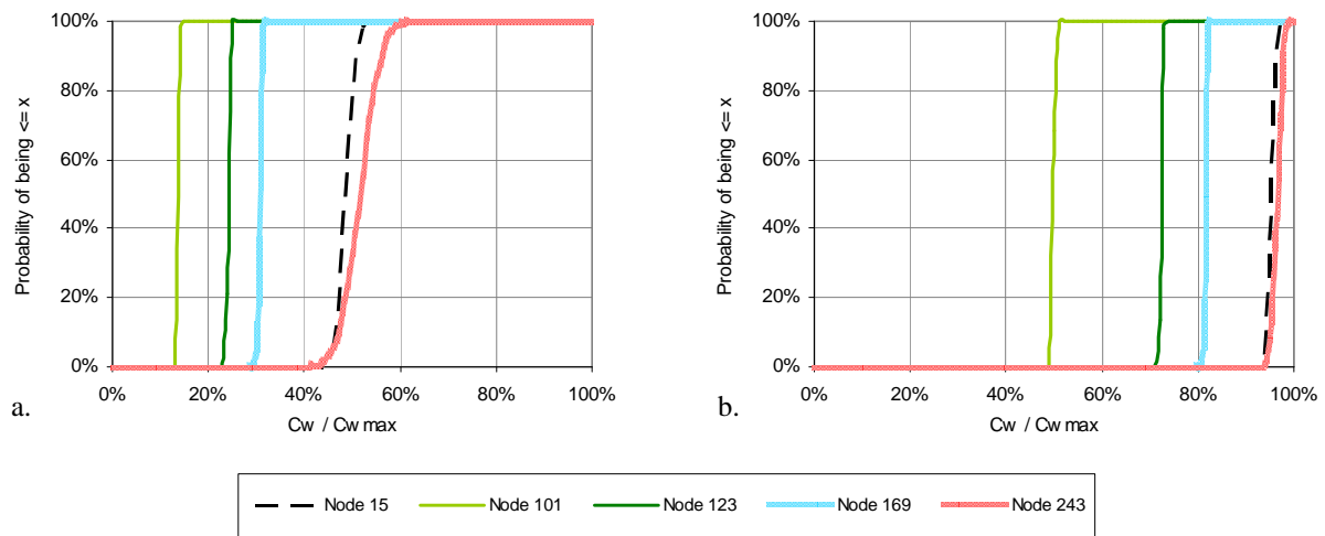
Figure 36 Simulation results for “Net 3”: cumulative distribution of the migrant concentration The two graphs represent the probability distribution that the saturation level along the day is \leq x (the abscissa), for migrant’s diffusion coefficient in the water of 10^{-10} \text{ m}^2/\text{s} for Graph a and 10^{-9} \text{ m}^2/\text{s} for Graph b. If one considers antioxidants such as Irganox 1010 or Irgafos 168 then the concentration of species in the PE matrix is about 2 g/kg and their partition coefficient at the interface around 1.55 \cdot 10^{-4} , leading to a saturation concentration of 310 \mu\text{g}/\text{L} .
