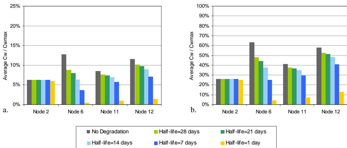
Figure 17 Simulation results for the Farum network: effect of degradation on the migrant concentration The figure represents the daily average of the migrant saturation level at relevant nodes of the network and for different migrant half-lives. In these simulations, the migrant's diffusion coefficient in the water is 10^{-10} m 2 /s for Graph a and 10^{-9} m 2 /s for Graph b. If one considers antioxidants such as Irganox 1010 or Irganox 168 then the concentration of species in the PE matrix is about 2 g/kg and their partition coefficient at the interface around 1.55 \cdot 10^{-4} , leading to a saturation concentration of 310 µg/L.
