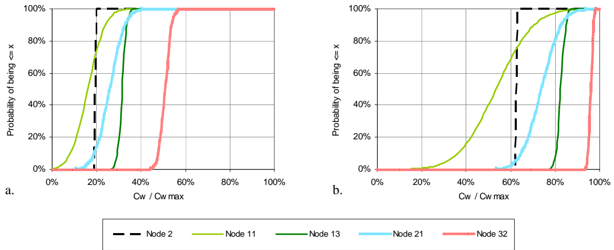
Figure 27 Simulation results for “Net 1”: cumulative distribution of the migrant concentration The two graphs represent the probability distribution that the saturation level along the day is \leq x (the abscissa), for migrant’s diffusion coefficient in the water of 10^{-10} \text{ m}^2/\text{s} for Graph a and 10^{-9} \text{ m}^2/\text{s} for Graph b. If one considers antioxidants such as Irganox 1010 or Irgafos 168 then the concentration of species in the PE matrix is about 2 g/kg and their partition coefficient at the interface around 1.55 \cdot 10^{-4} , leading to a saturation concentration of 310 \mu\text{g/L} .
