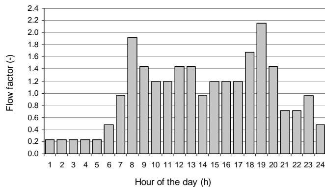
Figure 7 Flow factors used in EPANET to simulate diurnal variations in demand At every time step, the actual demand is obtained by multiplying the base demand by the corresponding multiplier.
