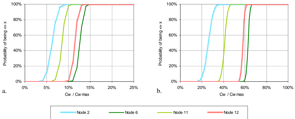
Figure 16 Simulation results for the Farum network: cumulative distribution of the migrant concentration The two graphs represent the probability distribution that the saturation level along the day is \leq x (the abscissa), for migrant’s diffusion coefficient in the water of 10^{-10} \text{ m}^2/\text{s} for Graph a and 10^{-9} \text{ m}^2/\text{s} for Graph b. If one considers antioxidants such as Irganox 1010 or Irgafos 168 then the concentration of species in the PE matrix is about 2 g/kg and their partition coefficient at the interface around 1.55 \cdot 10^{-4} , leading to a saturation concentration of 310 \mu\text{g/L} .
