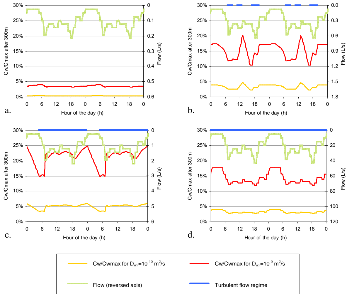
Figure 8 EPANET dynamic simulations on a single pipe Graph a, b, c, d represent simulation results for a base flow of 0.1 L/s, 0.3 L/s, 1 L/s, and 20 L/s, respectively. Each graph displays the computed saturation level in migrant at the outlet of a pipe of 200 mm diameter and 300 m length. The flow is shown using a secondary axis which has been reversed to highlight similarities between flow and migrants content. A binary representation is used to display the flow regime: if there is a blue line the flow is turbulent, otherwise it is laminar. Simulations are made for two cases of migrant's diffusion coefficient in the water: 10^{-10} and 10^{-9} m^2/s . If one considers antioxidants such as Irganox 1010 or Irgafos 168 then the concentration of species in the PE matrix is about 2 g/kg and their partition coefficient at the interface around 1.55 \cdot 10^{-4} , leading to a saturation concentration of 310 \mu g/L .
