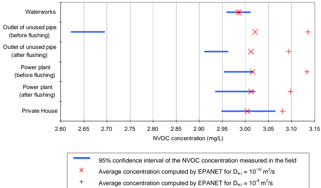
Figure 20 Comparison between modelling and sampling results for the Farum network. The modelling results correspond to the antioxidants Irganox 1010 or Irgafos 168, which have a concentration in the PE matrix of about 2 g/kg and a partition coefficient at the interface around 1.55 \cdot 10^{-4} , leading to a saturation concentration of 310 \mu\text{g/L} .
