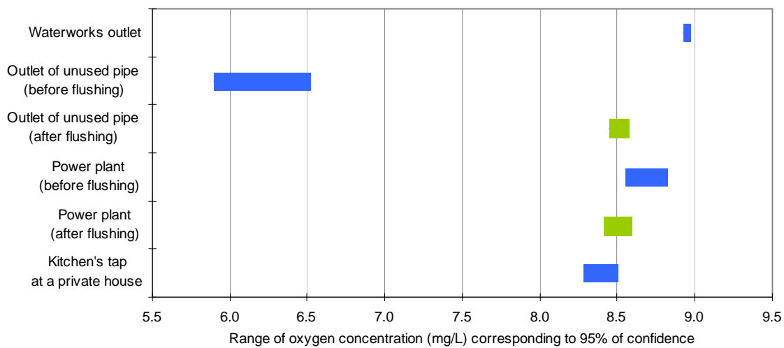
Figure 19 95% confidence interval of the oxygen concentration measured in the Farum network on 29/04/08 A colour code distinguishes the concentrations measured after flushing (light green) from the others (dark blue), which are assumed to reflect normal conditions in the network.
