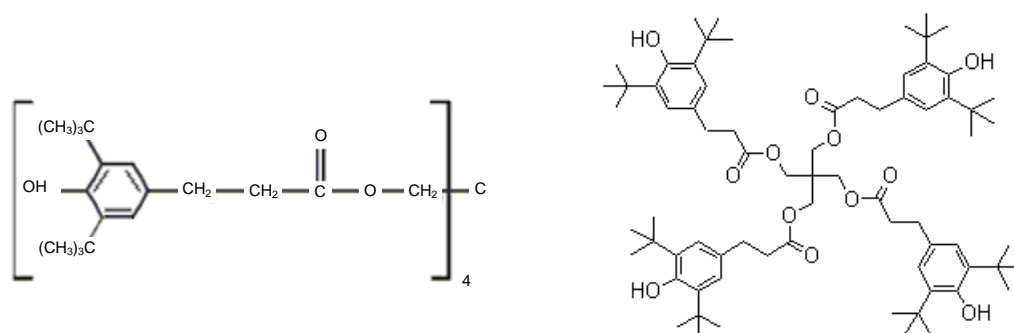
Figure 1 Molecular structure of the antioxidant Irganox 1010 From left to right, the displays are from Water Panel (2004) and ChemBlink (2008), respectively. Compound's chemical name: Tetrakis(3-(3,5-di-tert-butyl-4-hydroxyphenyl)propionate) Compound's CAS number: 6683-19-8
