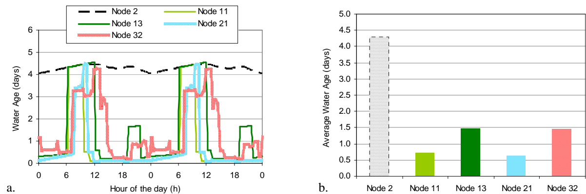
Figure 23 Computation of the water age in “Net 1” Graphs a and b represent respectively the water age variation along the day and its average value at relevant nodes of the network.
