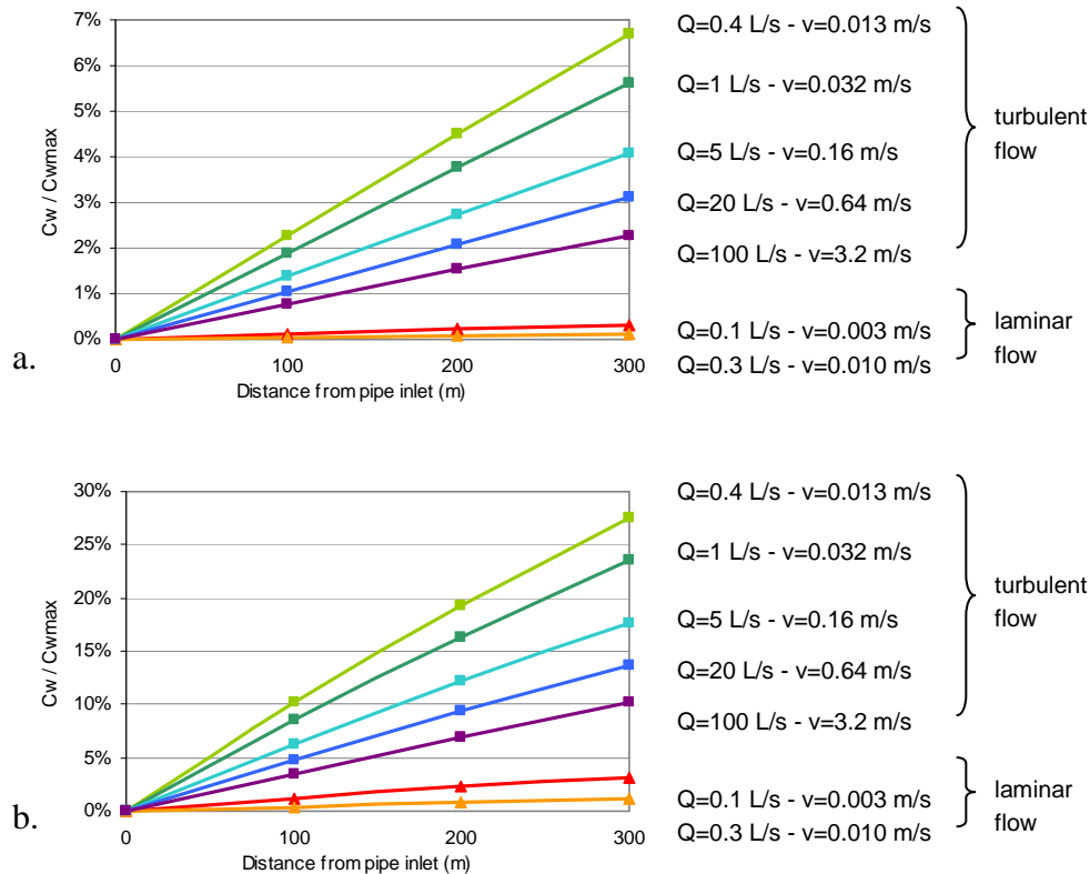
Figure 6 EPANET static simulations on a single pipe model The figure presents the migrant saturation level in the water computed along a pipe of 200 mm diameter. The charts illustrate the distribution along the pipe and the flow dependency. Chart a and b correspond to a diffusion coefficient of the species in the water of 10^{-10} m 2 /s and 10^{-9} m 2 /s, respectively. It should be noted that the ordinate scale is different between the two charts. If one considers antioxidants such as Irganox 1010 or Irgafos 168 then the concentration of species in the PE matrix is about 2 g/kg and their partition coefficient at the interface around 1.55 \cdot 10^{-4} , leading to a saturation concentration of 310 \mu g/L.
