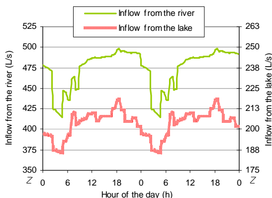
Figure 30 Computation of the inflow of water from the sources to the network in “Net 3” It should be noted that the two curves do not have the same Y axis. The inflow from the river is indeed quite higher.
