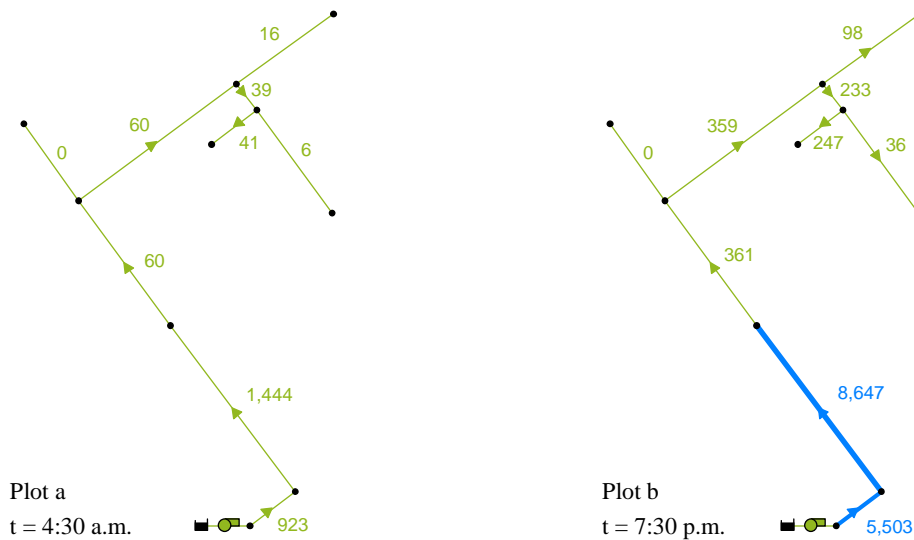
Figure 13 Computation of the Reynolds number in the Farum network The numbers plotted next to the pipes are estimations of the Reynolds number. The colour code indicates the distinction between laminar (thin green line) and turbulent (thick blue line) flow conditions.
