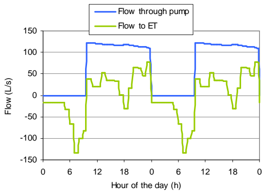
Figure 22 Computation of the waterworks pump working cycle in “Net 1”
