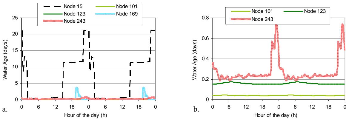
Figure 31 Computation of the water age in “Net 3”: variations along the day
