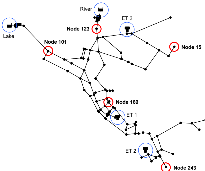
Figure 29 Sketch of the EPANET network model “Net 3” The thick-red circles indicate the locations that were considered relevant to give an overview of the pollution level. At these locations, the migrant concentration is analysed in detail. The thin-blue circles are used to highlight the locations of the two sources and the three elevated tanks (ET).
