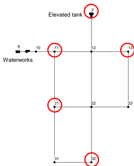
Figure 21 Sketch of the EPANET network model “Net 1” The red circles indicate the locations that were considered relevant to give an overview of the pollution level. At these locations, the migrant concentration is analysed in detail.
