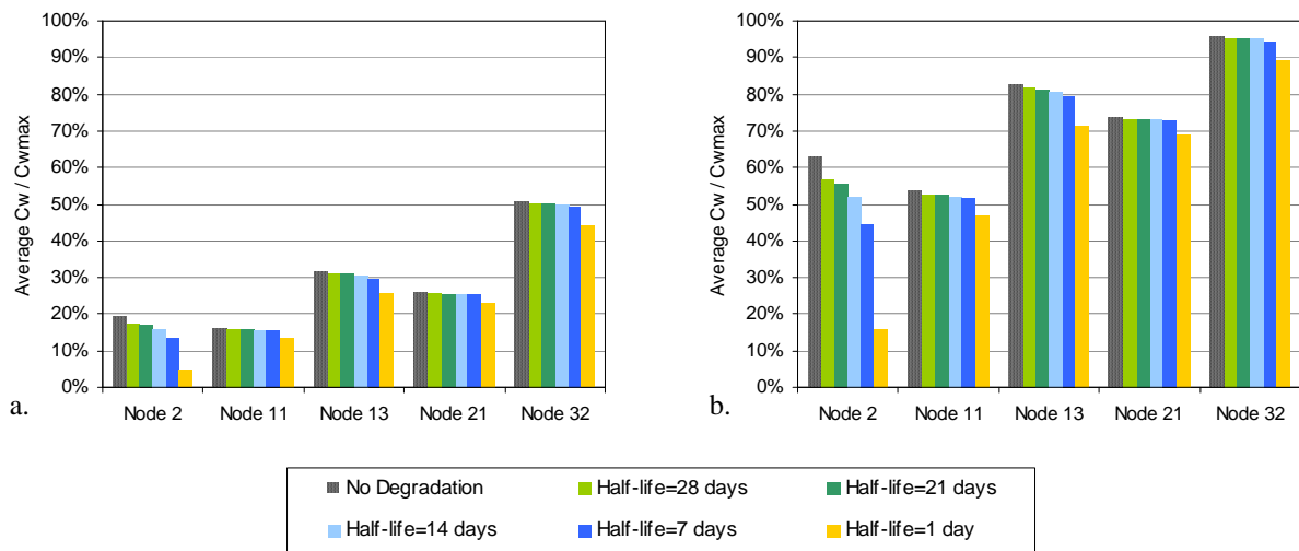
Figure 28 Simulation results for “Net 1”: effect of degradation on the migrant concentration The figure represents the daily average of the migrant saturation level at relevant nodes of the network and for different migrant half-lives. In these simulations, the migrant's diffusion coefficient in the water is 10^{-10} \text{ m}^2/\text{s} for Graph a and 10^{-9} \text{ m}^2/\text{s} for Graph b. If one considers antioxidants such as Irganox 1010 or Irganox 168 then the concentration of species in the PE matrix is about 2 g/kg and their partition coefficient at the interface around 1.55 \cdot 10^{-4} , leading to a saturation concentration of 310 \mu\text{g/L} .
