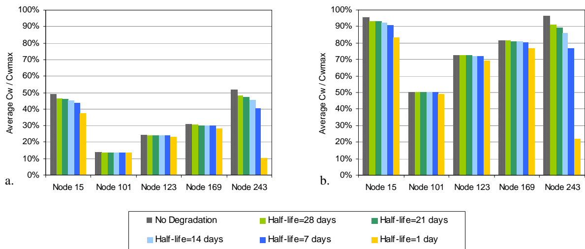
Figure 37 Simulation results for “Net 3”: effect of degradation on the migrant concentration The figure represents the daily average of the migrant saturation level at relevant nodes of the network and for different migrant half-lives. In these simulations, the migrant's diffusion coefficient in the water is 10 -10 m 2 /s for Graph a and 10 -9 m 2 /s for Graph b. If one considers antioxidants such as Irganox 1010 or Irgafos 168 then the concentration of species in the PE matrix is about 2 g/kg and their partition coefficient at the interface around 1.55*10 -4 , leading to a saturation concentration of 310 µg/L.
