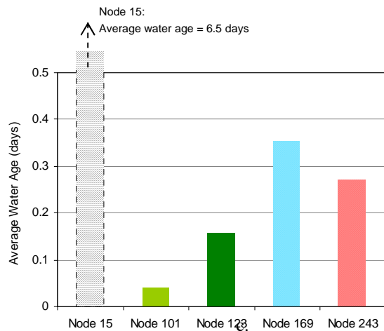
Figure 32 Computation of the water age in “Net 3”: mean age
