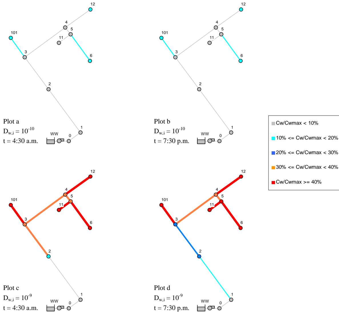
Figure 15 Simulation results for the Farum network: map-plot of the migrant concentration The figure represents the migrant saturation level in the network when no degradation is simulated at two times of the day. Plots a and b correspond to the case where a diffusion coefficient of the migrants in the water is 10^{-10} \text{ m}^2/\text{s} , and plots c and d to the case where it is 10^{-9} \text{ m}^2/\text{s} . If one considers antioxidants such as Irganox 1010 or Irgafos 168 then the concentration of species in the PE matrix is about 2 g/kg and their partition coefficient at the interface around 1.55 \cdot 10^{-4} , leading to a saturation concentration of 310 \mu\text{g}/\text{L} .
