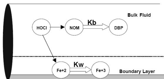
Figure 4 EPANET model: scheme of the reactions zones within a pipe
