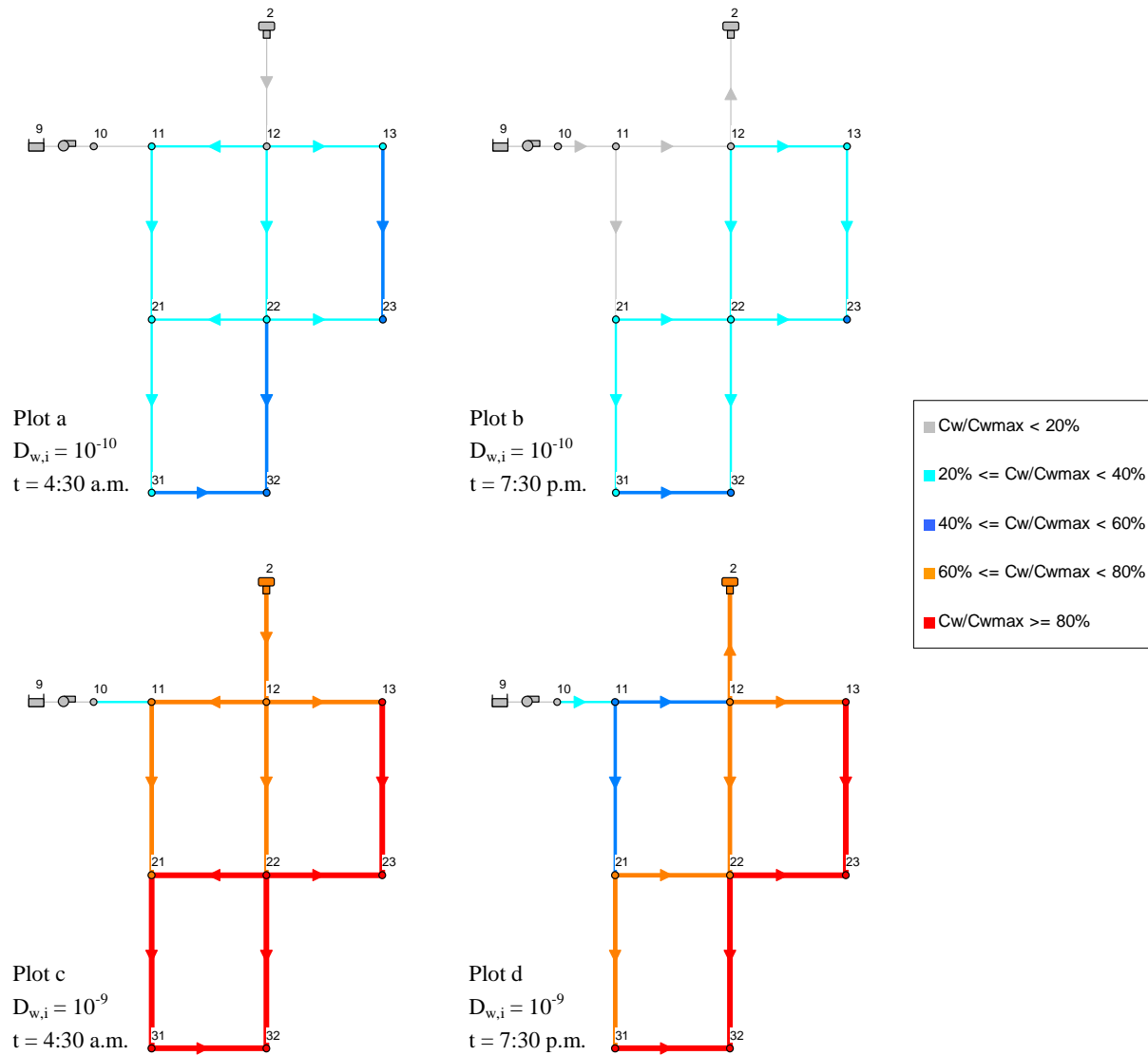
Figure 26 Simulation results for “Net 1”: map-plot of the migrant concentration
