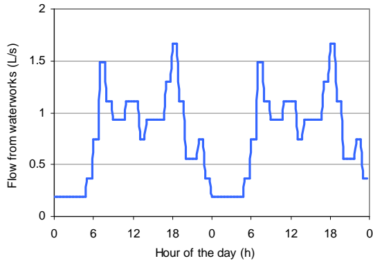
Figure 11 Computation of the flow sent from the waterworks to the Farum network
