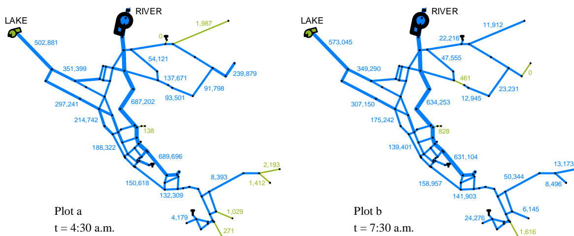
Figure 33 Computation of the Reynolds number in the “Net 3” The numbers plotted next to the pipes are estimations of the Reynolds number. The colour code indicates the distinction between laminar (thin green line) and turbulent (thick blue line) flow conditions.
