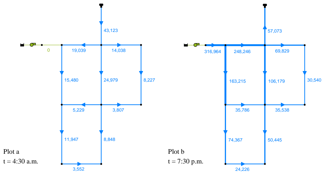
Figure 24 Computation of the Reynolds number in “Net 1” The numbers plotted next to the pipes are estimations of the Reynolds number. The colour code indicates the distinction between laminar (thin green line) and turbulent (thick blue line) flow conditions.
