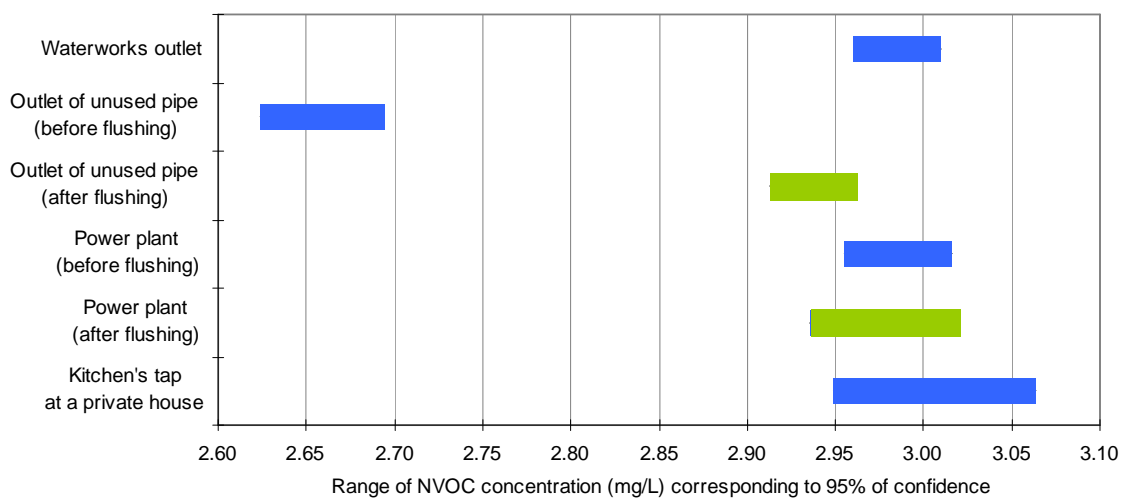
Figure 18 95% confidence interval of the NVOC concentration measured in the Farum network on 29/04/08 A colour code distinguishes the concentrations measured after flushing (light green) from the others (dark blue), which are assumed to reflect normal conditions in the network.
