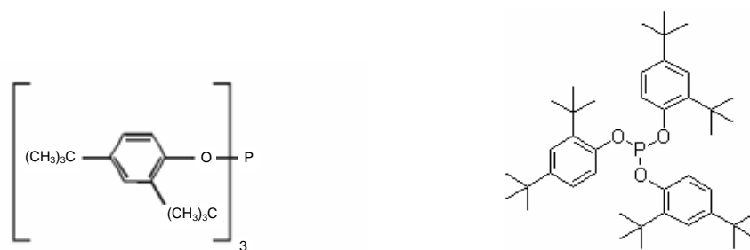
Figure 2 Molecular structure of the antioxidant Irgafos 168 From left to right, the displays are from Water Panel (2004) and ChemBlink (2008), respectively. Compound's chemical name: Tris(2,4-ditert-butylphenyl)phosphite Compound's CAS number: 31570-04-4
