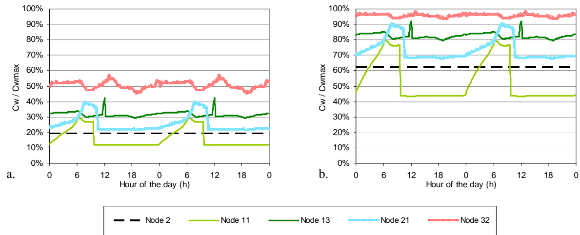
Figure 25 Simulation results for “Net 1”: daily variations of the migrant concentration The two graphs represent the saturation level of species along the day at relevant nodes of the network, for migrant’s diffusion coefficient in the water of 10^{-10} m 2 /s for Graph a and 10^{-9} m 2 /s for Graph b. If one considers antioxidants such as Irganox 1010 or Irgafos 168 then the concentration of species in the PE matrix is about 2 g/kg and their partition coefficient at the interface around 1.55 \cdot 10^{-4} , leading to a saturation concentration of 310 µg/L.
