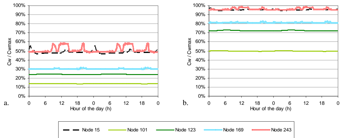
Figure 34 Simulation results for “Net 3”: daily variations of the migrant concentration The two graphs represent the saturation level of species along the day at relevant nodes of the network, for migrant’s diffusion coefficient in the water of 10^{-10} m 2 /s for Graph a and 10^{-9} m 2 /s for Graph b. If one considers antioxidants such as Irganox 1010 or Irgafos 168 then the concentration of species in the PE matrix is about 2 g/kg and their partition coefficient at the interface around 1.55 \cdot 10^{-4} , leading to a saturation concentration of 310 µg/L.
