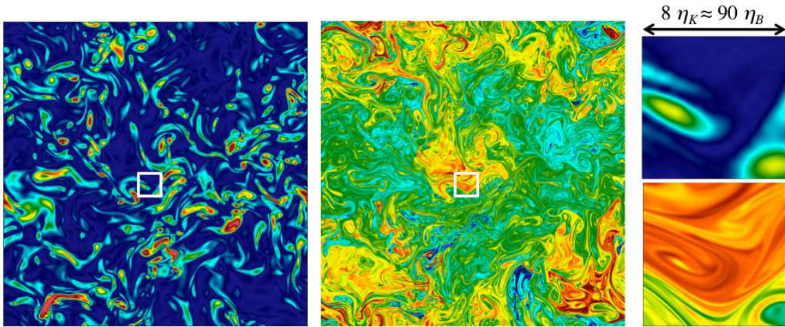
FIGURE 1. Vorticity (left) and scalar (middle) scales in a turbulent flow. Schmidt number=128. Right pictures : zoom of flow and scalar showing the scale gap between the vorticity (top) and the scalar (bottom).
