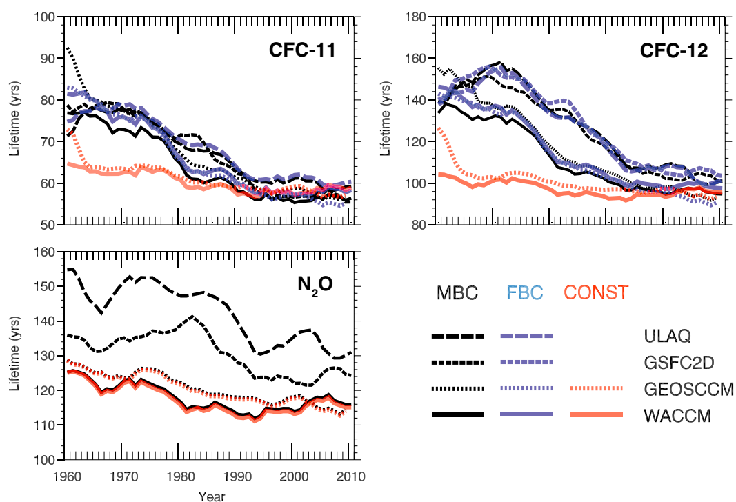
Figure 5. Time evolution of modeled atmospheric lifetimes of MBC CFC-11, CFC-12, and N_2O (black lines) between 1960 and 2010 from the TRANS simulations and their corresponding FBC (blue lines) and CONST (red lines) tracers when available. For clarity, the lifetimes are smoothed with a 5 year running mean filter.
