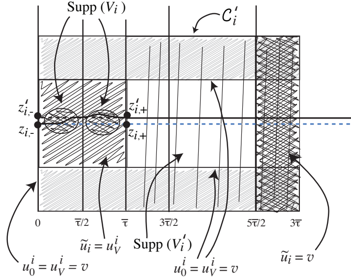
Figure 2: The curve \Gamma_i corresponds to the horizontal segment starting from the point z_{i,+}^i and going to the right. The function \tilde{u}_i is obtained by interpolating (using a cut-off function) between u_V^i (the viscosity solution for H_V ) and v (the critical subsolution for H constructed in Section 3.3.3) inside the “cylinder” C_i' . Then, by adding a new potential V_i' , small in C^2 topology and supported inside C_i' \cap \{z = (z_1, \hat{z}) \mid z_1 \in [\bar{\tau}, 3\bar{\tau}]\} , we can ensure that H_{V_i+V_i'}(z, \nabla \tilde{u}_i(z)) \leq 0 . Since the cylinders C_i' are disjoint, we can repeat this construction for i = 1, \dots, \eta - 1 to find a global critical subsolution \tilde{u} and a potential \tilde{V} so that (P1) and (P2) hold.
