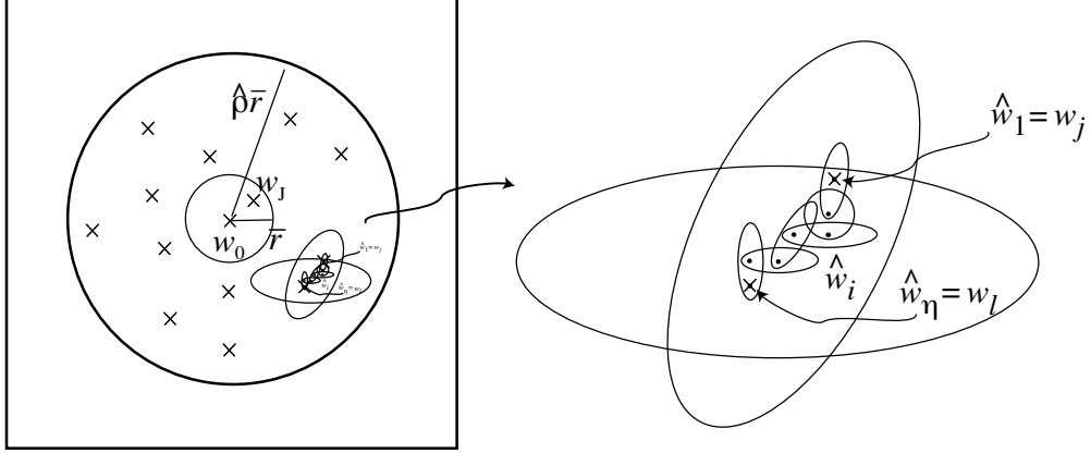
Figure 4: An illustration of Mai Lemma: there exist two points w_j, w_l , which can be connected using a sequence of \eta - 1 small ellipsoids E_i(\hat{w}_i, \hat{r}_i/\tilde{N}) , so that none of the points w_k ( k \neq j, l ) belongs to E_i(\hat{w}_i, \hat{r}_i) for i = 1, \dots, \eta - 1 (in the figure above, we just drew two of the ellipsoids E_i(\hat{w}_i, \hat{r}_i) ).
