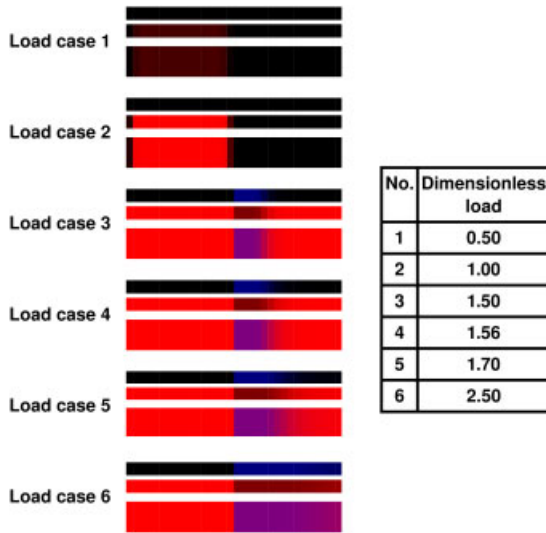
Fig. 6 (online colour at: www.zamm-journal.org ) Investigation of the influence of a value of parameter D introduced to account for the range of impact of osteocytes on the actor cells. The case of small value of D : the final configurations of a rod initially composed of two sub-domain occupied by bone tissue and by bio-material for different levels of mechanical external loading.
