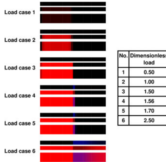
Fig. 7 (online colour at: www.zamm-journal.org ) Investigation of the influence of a value of parameter D introduced to account for the range of impact of osteocytes on the actor cells. The case of big value of D - the final configurations of a rod initially composed of two sub-domain occupied by bone tissue and by bio-material for different levels of mechanical external loading. It can be observed that for big values of D associated with a small domain of impact of osteocytes for most loading cases a void or very porous material appears in a domain initially occupied by the bone-substitute bio-resorbable material.
