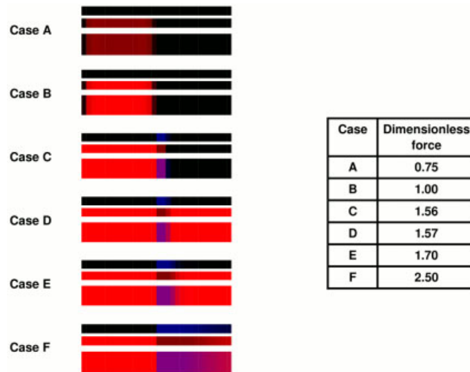
Fig. 5 (online colour at: www.zamm-journal.org ) The final configurations of a rod initially composed of two sub-domain occupied by bone tissue and by bio-material for different levels of mechanical external loading. The values of dimensionless load levels for the cases A-F are collected in a table at the right hand side of a figure.
