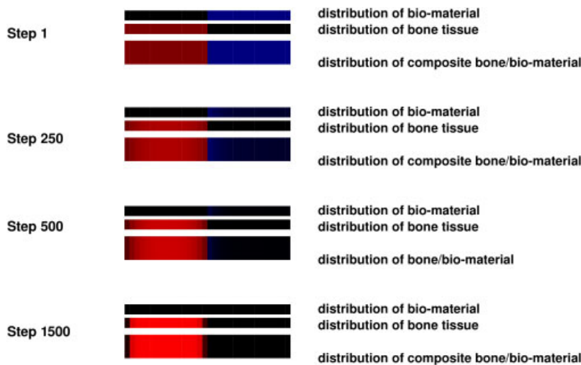
Fig. 3 (online colour at: www.zamm-journal.org ) Time evolution of material density distribution along the length of a rod initially composed of two rods, one made of bone tissue the other made of bio-resorbable bone-substitute material. The intensity of colours is proportional to the apparent densities of the materials. Thin bars display separately the distributions of bone tissue (red) and bone-substitute material (blue) and the thick bar reflects the sum of them the distribution of density of a composite bone tissue/bone-substitute material. The case of low level of the external load: significant resorption in a domain initially occupied by bio-material where the stimulus from the sensor cells is close to zero and formation of a very porous material can be observed.
