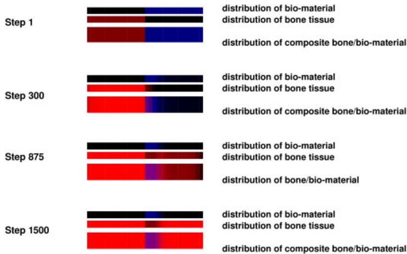
Fig. 4 (online colour at: www.zamm-journal.org ) Time evolution of material density distribution along the length of a rod initially composed of two rods, one made of bone tissue the other made of bio-resorbable bone-substitute material. The result of an analysis similar to the one displayed in Fig. 3 but for the case of relatively high level of the external load: a resorption in a domain initially occupied by bio-material is slower due to stronger stimulus from the sensor cells and formation of a new bone tissue in the pores present in bio-material can be observed. This process results in a partial replacement of bio-material by a natural tissue in some sub-domains and in formation of a composite bone/bio-material in others.
