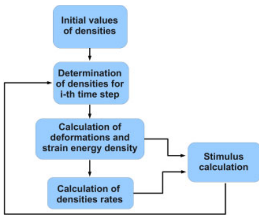
Fig. 2 (online colour at: www.zamm-journal.org ) A scheme of iterative numerical procedure used in an analysis of rod-bone remodeling in presence of bio-resorbable bone-substitute material.
