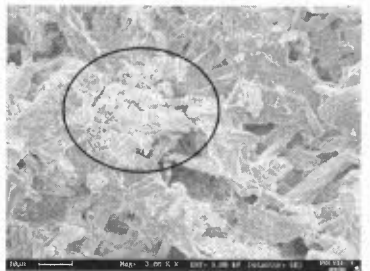
Fig. 5. Modification of the plaster phases versus temperature at 20, 100 and 300°C (DRX – SEM), G: gypsum, H: hemihydrate, A: anhydrite
