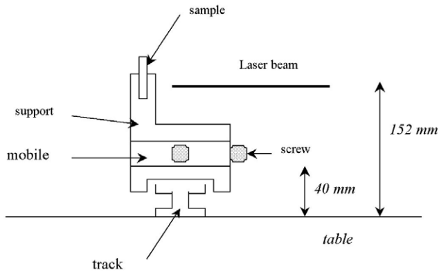
Fig. 3. Support for samples used at LPIO. The orientation of the laser beam is indicated as well as the movement direction of the support.
