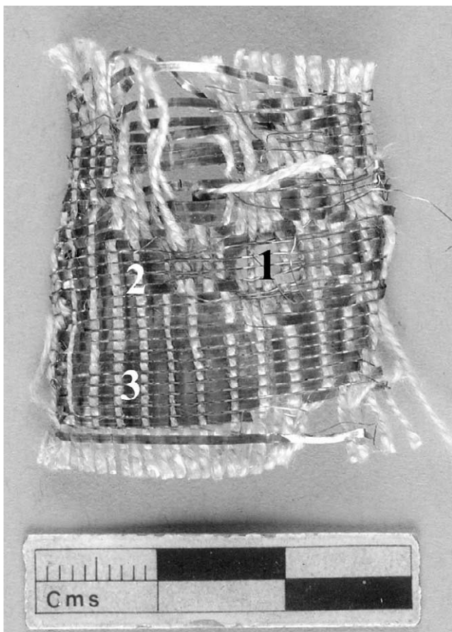
Fig. 10. Effect of laser cleaning with infrared radiation on a lace fragment with silvered copper threads under a flux of helium. 1: J = 1.43 \text{ J/cm}^2 and 10 impacts; 2: J = 0.43 \text{ J/cm}^2 and 10 impacts; 3: J = 0.43 \text{ J/cm}^2 and three impacts.
