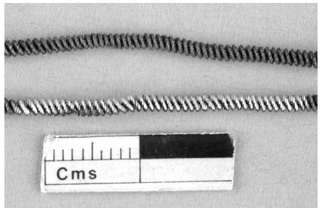
Fig. 11. Effect of laser cleaning with infrared radiation on gilt silver fringes from a flag. Top: uncleaned. The lower fringe was cleaned after several impacts ( J = 0.237 \text{ J/cm}^2 ).
