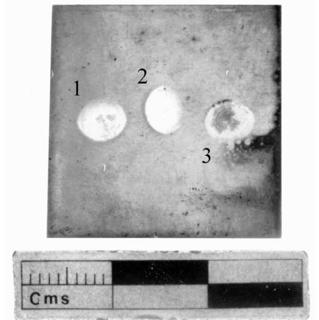
Fig. 5. Examples of laser impacts on an artificially sulphurised silver plate. In air, \lambda = 355 \text{ nm} ; 1 and 2: 10 pulses; 3: f = 10 \text{ Hz} for 40 s.
