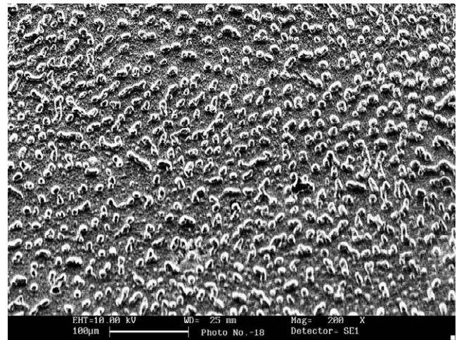
Fig. 6. Detail of an SEM picture showing the presence of prominent silver-based particles corresponding to the whitening phenomenon.
