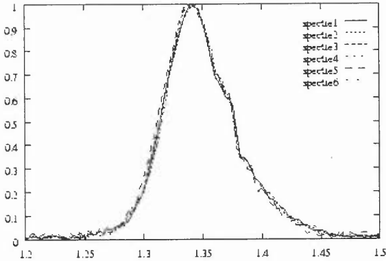
fig2 : LED spectra
