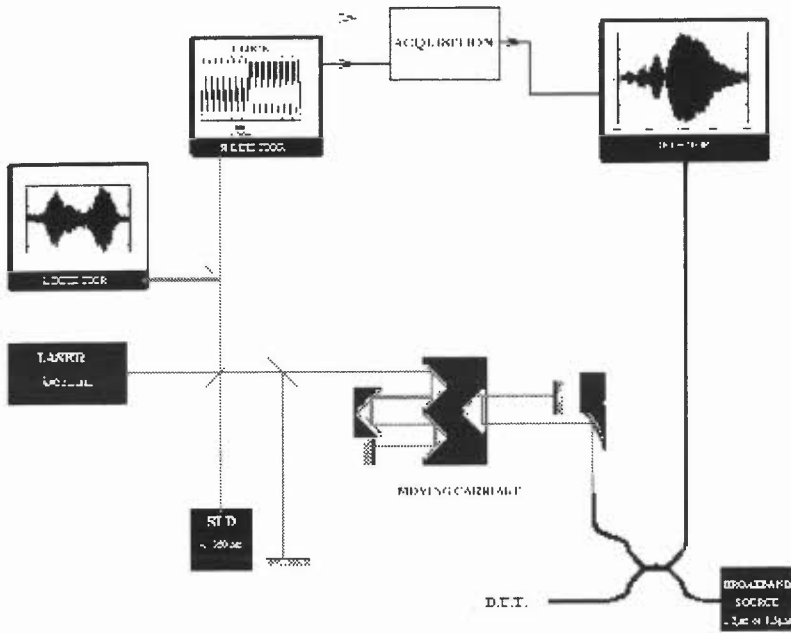
fig1 : experimental set-up
