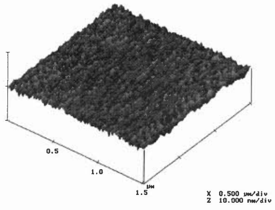
Figure 5: Image of the surface of 3 months at 85°C aged. fiber
