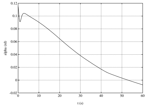
Fig. 7. Angle of attack \alpha (rad)
