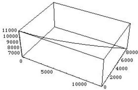
Fig. 1. Nonplanar dive
