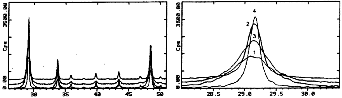
Fig. 3. X-ray diffraction pattern of Y_2O_3 , Y_2O_3:Eu samples annealed 600^\circ C in hour and standard sample: 1- Y_2O_3:Eu powder prepared with urea, 2- Y_2O_3:Eu powder prepared with G: M^{3+}=1.67 , 3- Y_2O_3 powder prepared with G: M^{3+}=1.67 , 4- Y_2O_3 standard sample
