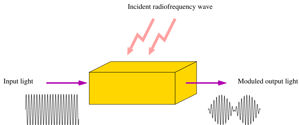
Figure 1. Electrooptic antenna
