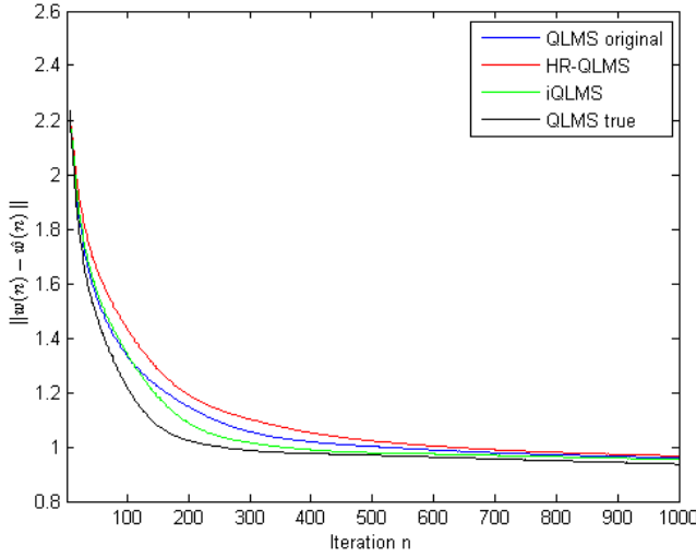
Fig. 2. Evolution of the estimation error \|w(n) - \hat{w}(n)\| as a function of the iteration n , averaged 100 times, for the original QLMS, the HR-QLMS, the iQLMS and the true QLMS.
