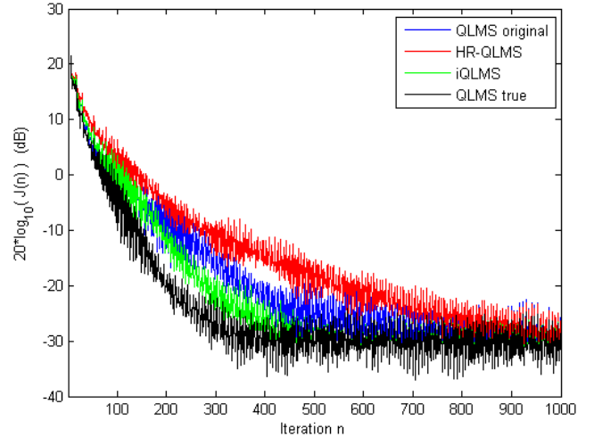
Fig. 1. Evolution of the criterion J(n) in dB as a function of the iteration n , averaged 100 times, for the original QLMS, the HR-QLMS, the iQLMS and the true QLMS.
