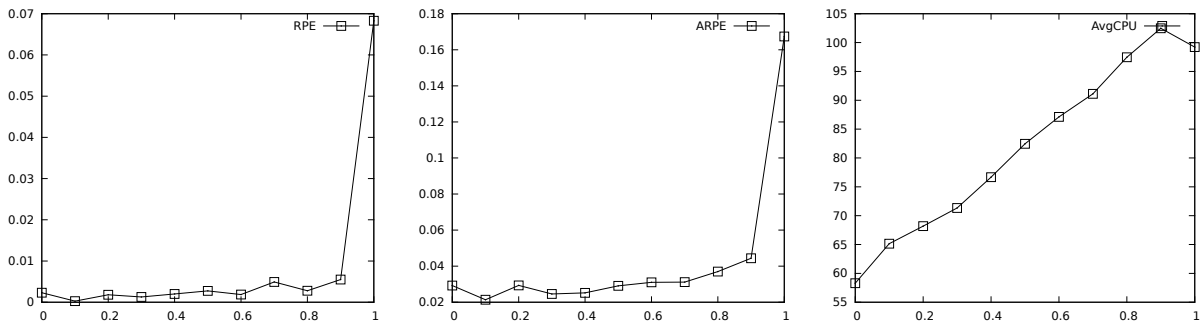
Figure 4: Performance of PSOiA in terms of the probability ph of a particle to be moved out of its current position.
