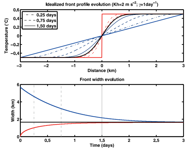
Figure 9. (top) Example of numerical temporal evolution of two idealized temperature fronts (linear gradient in blue; step-like in red) toward the analytical equilibrium profile (black) for a given combination of strain rate ( \gamma ) and eddy diffusivity ( K_H ). The numerical simulations were based on equation (1) using constant values of \gamma and K_H . The thinner lines mark intermediate front profiles at different times before the equilibrium. The red curve at 1.5 days coincides already with the analytical equilibrium profile (as shown in the bottom plot). (bottom) Temporal evolution of the widths of the linear gradient (blue) and step-like (red) fronts toward the width at the equilibrium (black). The width at the equilibrium was computed as W = 4\sigma . The gray lines mark the times corresponding to each intermediate profile plotted in the top plot. The figure indicates a relatively rapid adjustment (on the order of 1–2 days) of the front profile toward the equilibrium. Analogous results were obtained for various combinations of K_H and \gamma within the range of the observed values.
