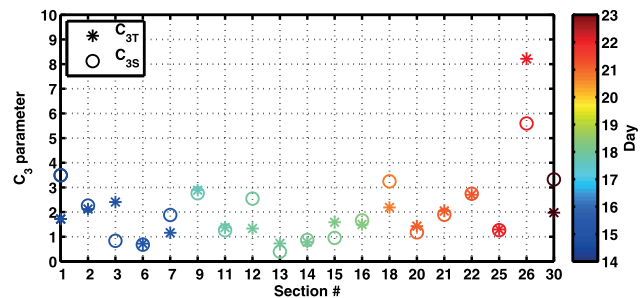
Figure 6. Values of the C_3 parameter from equation (3) estimated from each fitted profile of SST (stars) and SSS (circles) from Figure 5. As in Figure 5, the values are color coded according to the day each profile was collected.
