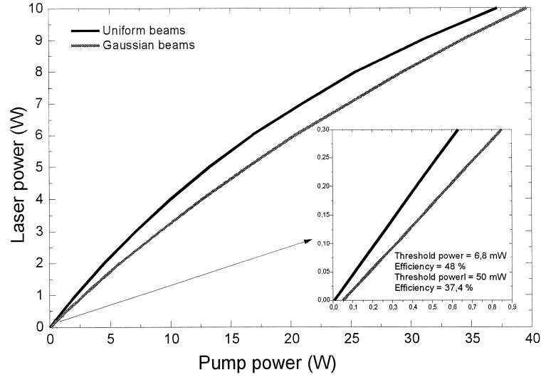
Fig. 2. Laser power versus pump power for uniform and Gaussian beams. No losses – R = 99\% – w_1 = w_p = 100 \mu\text{m} .
