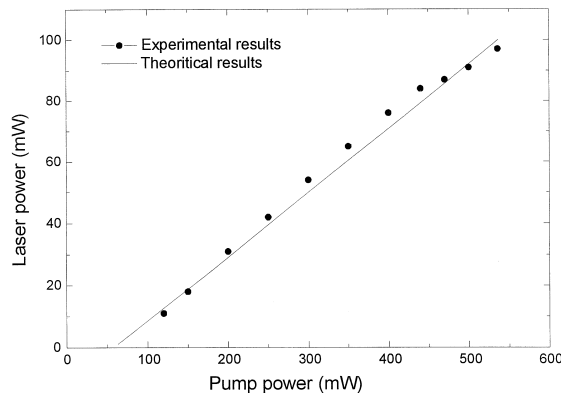
Fig. 3. Laser power versus pump power for experimental and theoretical pumping by a \text{Ti:Al}_2\text{O}_3 laser.
