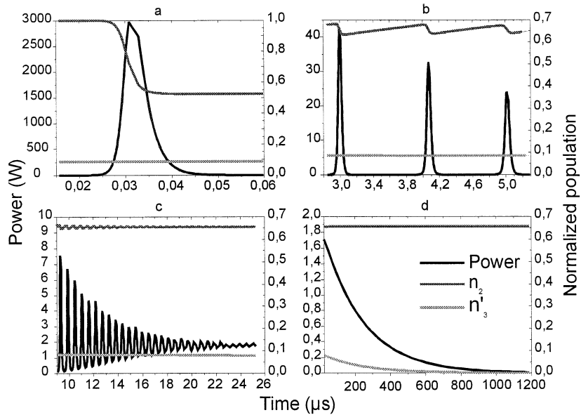
Fig. 7. Temporal evolution of the peak power and population of \text{Yb}^{3+} \ ^2F_{5/2} level and \text{Er}^{3+} \ ^4I_{13/2} level (time scales are different in the different graphs).
