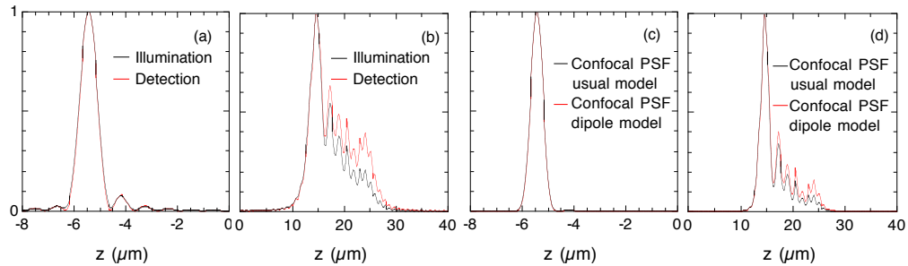
Fig. 2: Illumination and detection PSF at \lambda=488 nm with a 40x, N.A.=0.9 dry objective, for a single fluorescent molecule located in a watery medium 50 \mu\text{m} below (a): a 120 \mu\text{m} thickness cover glass and (b): a 170 \mu\text{m} thickness cover glass. (a) and (b) are for a conventional microscope. (c) and (d): confocal PSFs computed with the usual model and our dipole model. Figures (c) and (d) correspond to the same conditions as (a) and (b), respectively.
