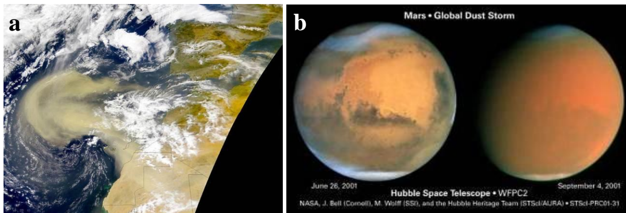
Figure 1.2. (a) Satellite image of a massive dust storm blowing off the northwest Sahara desert on February 26, 2000. Image credit: Visible Earth, NASA ( http://visibleearth.nasa.gov/ ). (b) Hubble space telescope images of roughly the same hemisphere of Mars, illustrating the effects of the 2001 planet-encircling dust storm. The left image was acquired on 26 June 2001 and shows the dust storm beginning at the lower right of the disk. The right image was acquired on 4 September 2001, and shows dust shrouding most of the planet. Image credit: NASA/James Bell (Cornell University)/Michael Wolff (Space Science Institute)/The Hubble Heritage Team (STScI/AURA).
