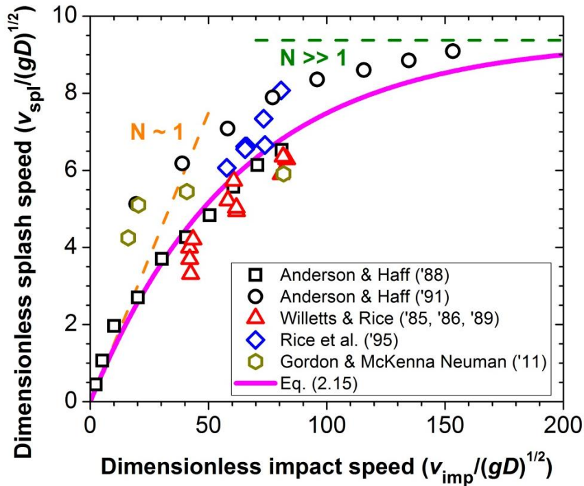
Figure 2.6. The average dimensionless speed of splashed surface particles ( \overline{v_{\text{spl}}} / \sqrt{gD} ) as a function of the dimensionless speed of the impacting particle ( v_{\text{imp}} / \sqrt{gD} ). Black and colored symbols respectively denote the results from numerical (Anderson and Haff 1988, 1991) and laboratory (Willetts and Rice 1985, 1986, 1989, Rice et al. 1995, 1996; Gordon and McKenna Neuman 2011) experiments with natural sand. The dashed orange and green lines show the limits at N \sim 1 (Eq. (2.12)) and N \gg 1 (Eq. (2.13)), respectively, and the magenta line denotes the prediction of Eq. (2.15). These relations used \alpha = 0.15 and a = 0.016 (Rice et al. 1995, Kok and Renno 2009a).
