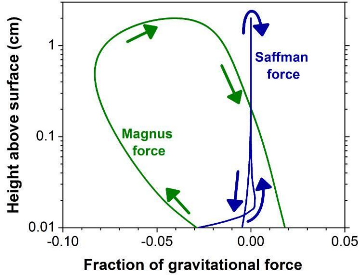
Figure 2.3. The Magnus force (green line) and the Saffman force (blue line) as a fraction of the gravitational force during the saltation trajectory of a 200\text{ }\mu\text{m} particle launched from the surface with a speed of 1\text{ m/s} at an angle of 40^\circ from horizontal and a rotational speed of 400\text{ rev/s} . The arrows indicate the direction of particle motion. The particle trajectory and lift forces were calculated using Eqs. 1 – 6 in Kok and Renno (2009a), using the vertical profile of the horizontal wind speed of Eq. (2.18) with u_* = 0.20\text{ m/s} and z_0 = D_p/30 . The asymmetries in the relative strength of both the Magnus and the Saffman force on the upward and the downward trajectories are due to changes in the velocity of the particle relative to the flow, which determines the strength and direction of these forces. The effects of turbulence were neglected.
