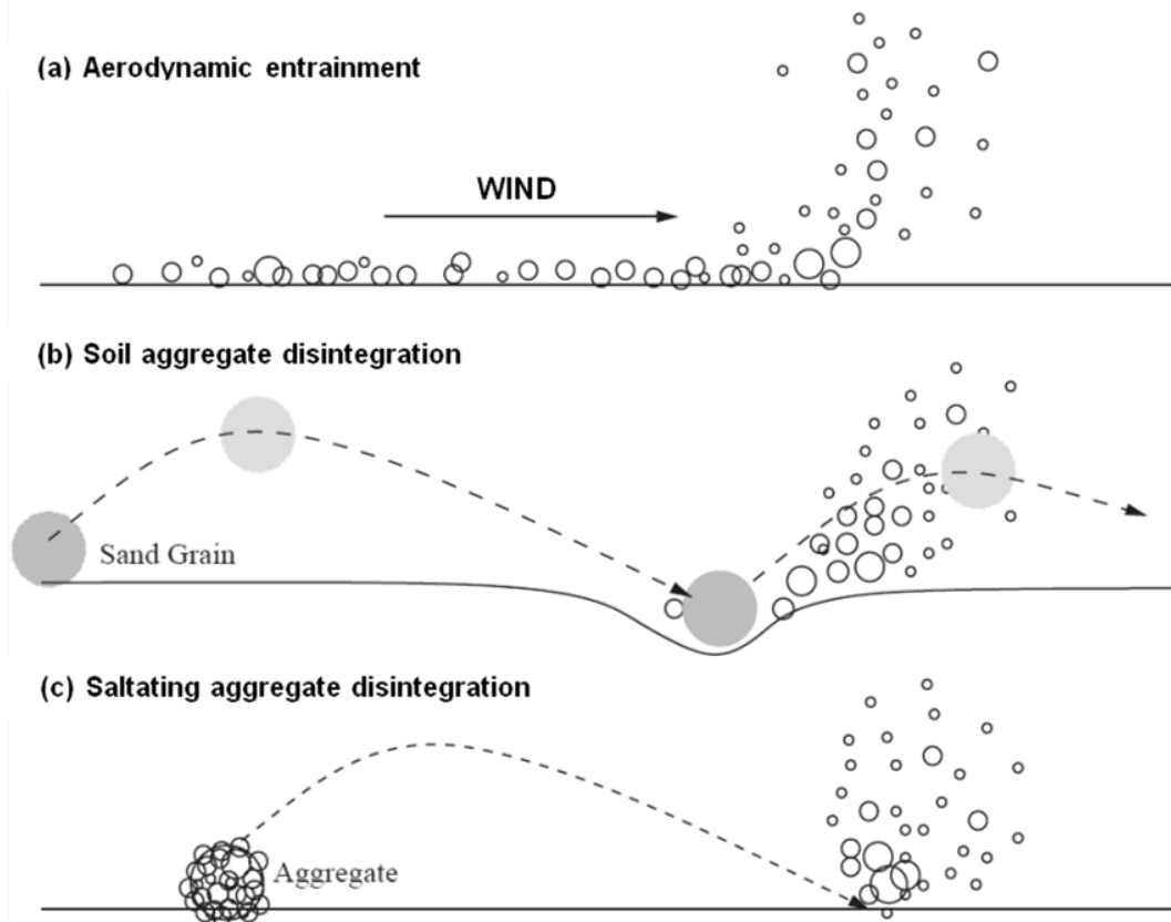
Figure 4.1. Illustration of the three dust emission mechanisms: (a) aerodynamic entrainment, (b) ejection of dust aerosols from soil aggregates by impacting saltating particles, and (c) ejection of dust aerosols from soil aggregates that are participating in saltation. Adapted from figure 7.5 in Shao (2008).
