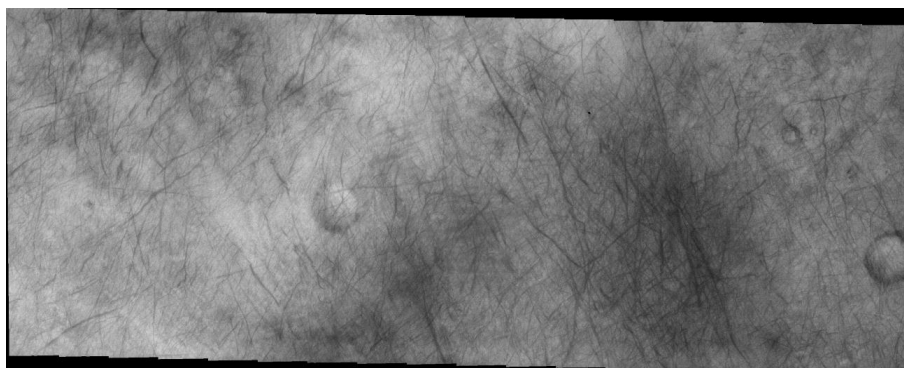
Figure 5.10. Example of orbitally observed dust devil tracks on Mars at \sim 69.5^\circ\text{S} (north is to the left; area of \sim 66 \times 20 km with a pixel size of \sim 19 m). Note the concentrations of dark dust devil tracks. Mars Odyssey THEMIS image V33501003 (Christensen et al. 2011).
