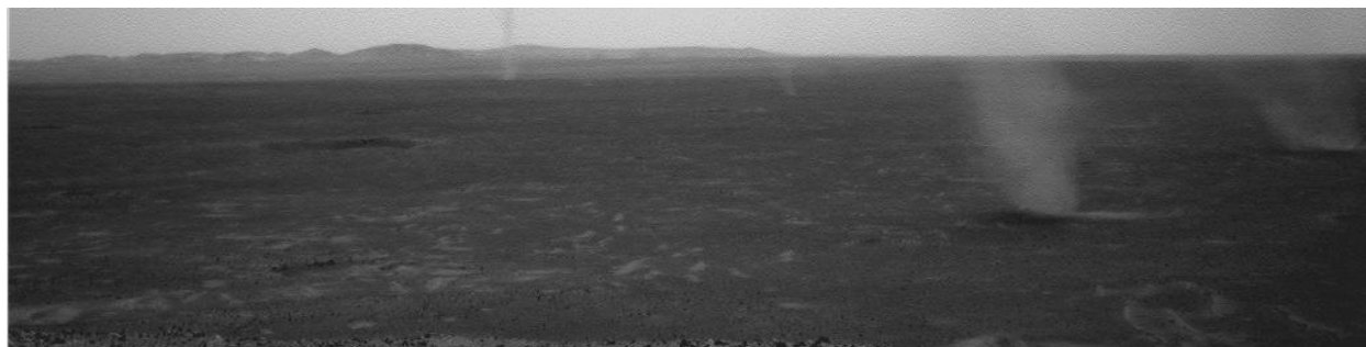
Figure 5.9. Mars Exploration Rover Spirit image from its Navigation Camera, showing multiple simultaneous smaller dust devils of different sizes and intensities. Acquired on Sol 568 within Gusev Crater, Mars. Image credit: NASA/JPL/Cornell/USGS
