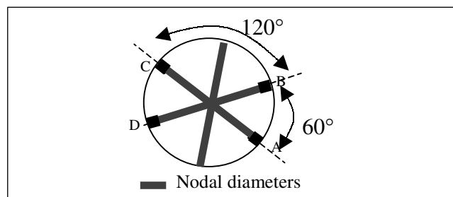
Fig. 10: Sinus mode (0,3)—Nodal diameter locations
