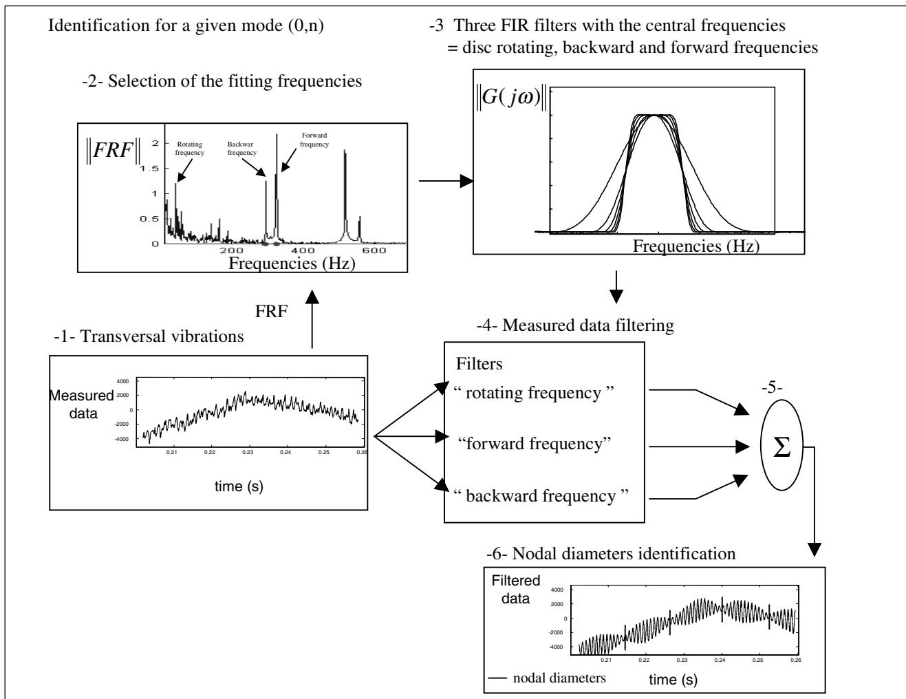
Fig. 3: Identification process for a given mode (0,n)
