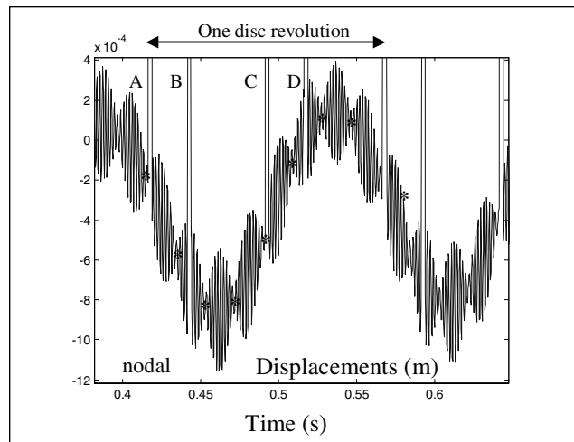
Fig. 9: Sinus mode (0,4)—Filtered time response
