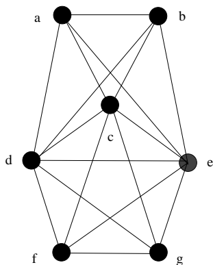
Figure 2: Forbidden component of a (K_5, k) stable graph with minimum size.
