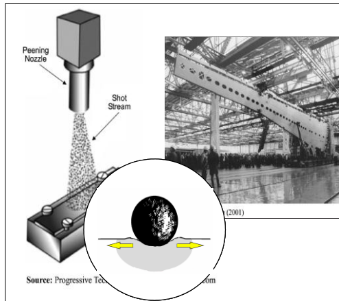
Figure 5: Illustration of the peen forming process.
