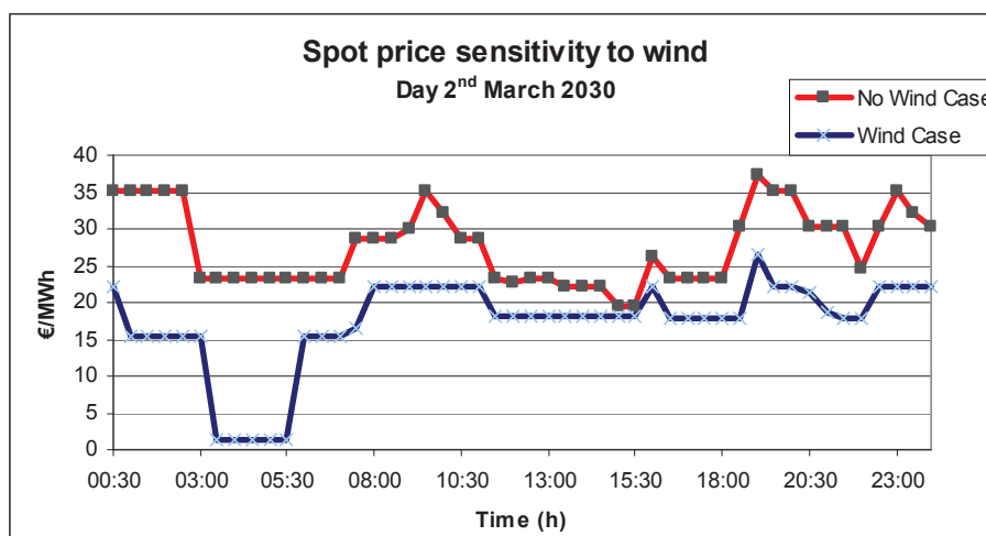
Fig. 3. Spot price difference in cases with and without wind, in the scenario GAS 2030
