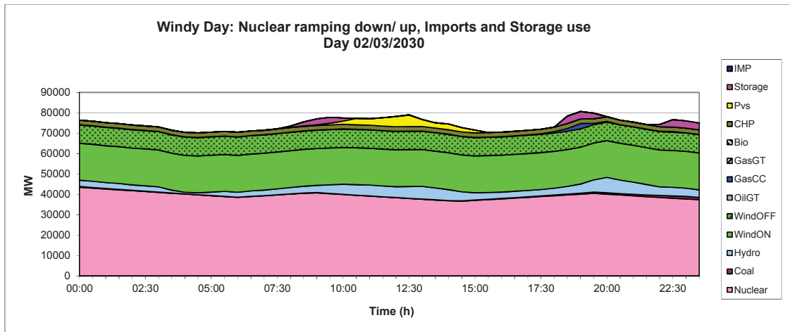
Fig. 1. Power plants dispatching during a windy day, scenario EC 2030
