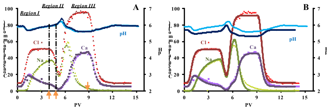
Fig. 1: Breakthrough curves obtained for pH and concentrations of aqueous Na, Ca and Cl reported as a function of the number of pore volumes (PV) injected in the column. Experimental results obtained at two different flow rates are reported on Fig. 1A while Fig. 1B compares experimental results (dot symbols) obtained at a flow rate of 6 mL/h with calculated BTC (lines) predicted by our model. The arrows indicate the injection of solutions having different chemistry as detailed in the text (section 3).
