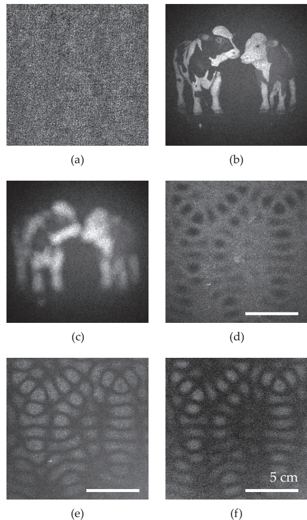
FIG. 3. Images of the cows : |\tilde{I}_1| (a), |H_1| at z = 0.47 m (b), |H_1| at z = 0.39 m (c). Contour modes of the plate vibrating at 21.5 kHz : |H_1| (d), |H_3| (e), and |H_3/H_1| (f).
