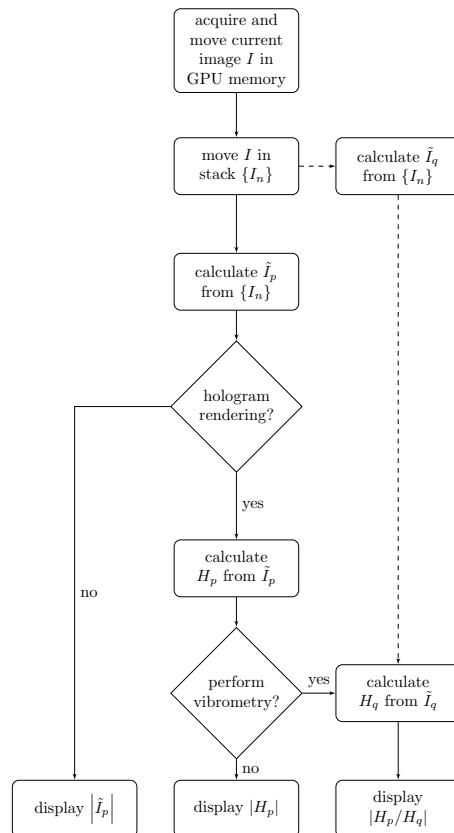
FIG. 1. Flow chart of holographic image acquisition, rendering and display. Raw interferograms are recorded by the acquisition thread. Temporal and spatial signal demodulation are performed by the hologram rendering thread. Image display is performed by a separate thread.
