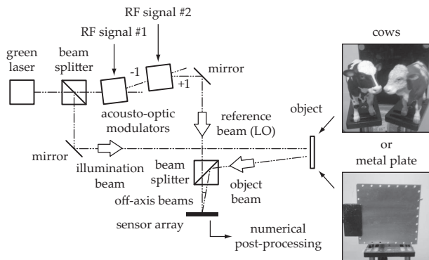
FIG. 2. Optical arrangement. The main laser beam is split into two channels, forming a Mach-Zehnder interferometer. The probe beam is backscattered by an object, yielding the optical field E . In the reference channel, the optical local oscillator field E_{LO} is frequency-shifted by two acousto-optic modulators, driven by phase-locked frequency synthesizers, from which alternate diffraction orders ( \pm 1 ) are selected. Holographic images are computed numerically from interferometric measurements of the diffracted object beam beating against the local oscillator beam.
