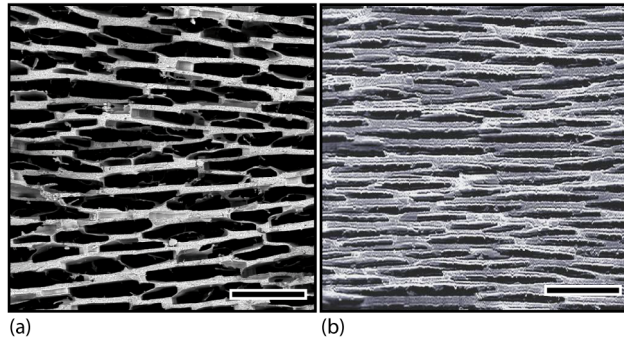
FIG. 3: Ice-templated alumina obtained with (a) a 50% coke/50% water solvent (b) citric acid and sugar addition in water. Scale bars: (a) 100 microns (b) 200 microns.
