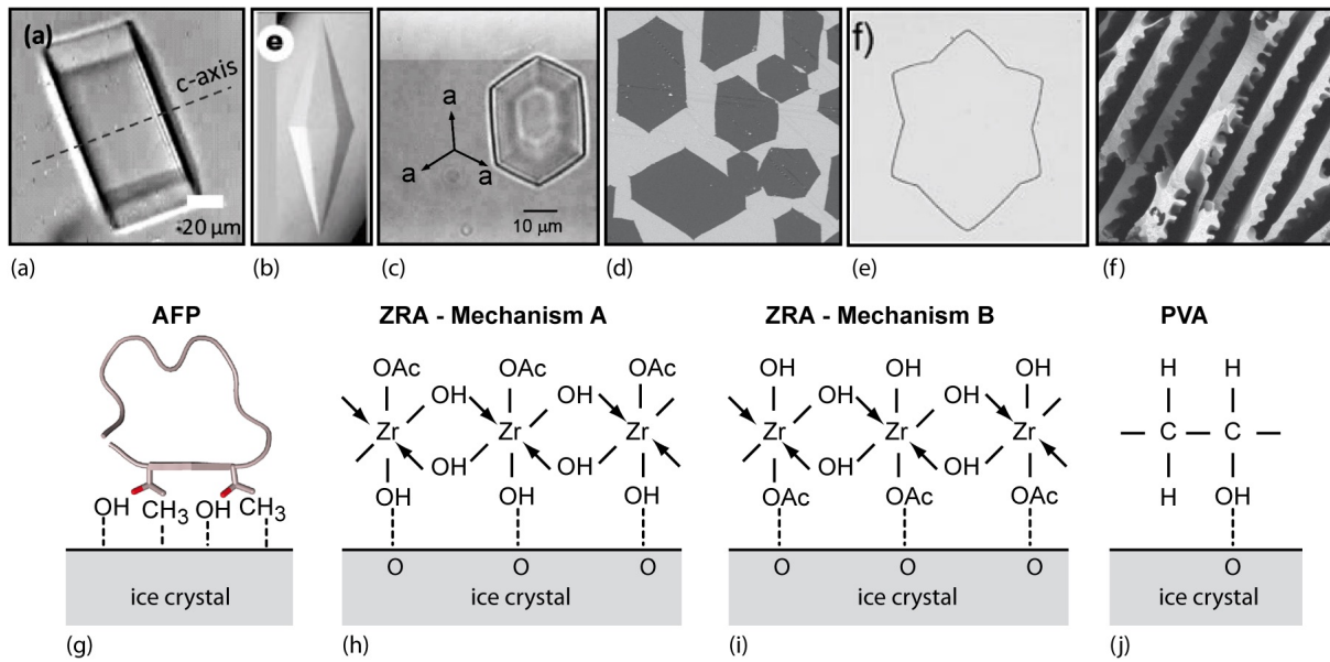
FIG. 9: Ice crystals and ice-templated pores in presence of ice-structuring proteins and compounds, and corresponding mechanisms of interaction with the crystal surface. (a) Ice crystals in presence of antifreeze glycoproteins analogue. Reprinted (adapted) with permission from 159 . Copyright (2010) American Chemical Society. (b) Ice crystals in presence of fish type I AFP from the winter flounder. Copyright (2000) Nature Publishing Group. Used with permission from 160 . (c) Ice crystals in presence of \beta -helical antifreeze protein from Tenebrio molitor . Reprinted (adapted) with permission from 161 . Copyright (2008) American Chemical Society. (d) Ice templated pores in 8Y-TZP in presence of ZRA. (e) Ice crystals in presence of PVA. Copyright (2007) Wiley. Used with permission from 130 . (f) Ice templated pores in alumina in presence of PVA. (g) Adapted from 129 .
