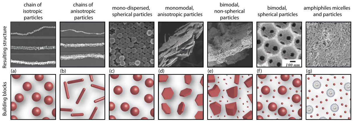
FIG. 5: Assembly and self-assembly of isotropic and anisotropic building blocks induced by the growth of the surrounding ice crystals. Sources: (a, b) Reprinted (adapted) with permission from 78 . Copyright (2011) American Chemical Society (c) Frozen colloidal silica, micrograph by A. Bogner 155 (d, e) Copyright (2012) Elsevier. Used with permission from 76 (f) Reprinted (adapted) with permission from 28 . Copyright (2009) American Chemical Society (g) 85 . Color online.
