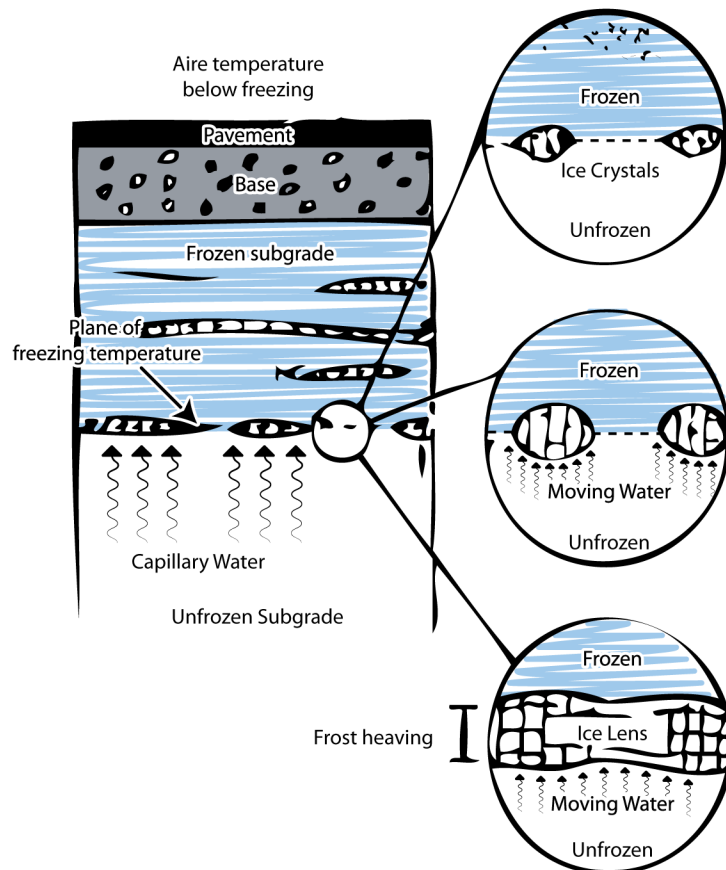
FIG. 6: Frost heave of a road, schematic representation. Adapted from 156 . Color online.
