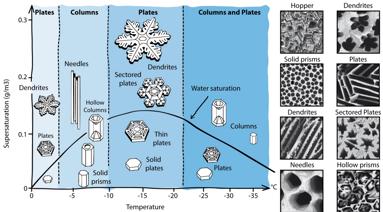
FIG. 4: Morphology diagram of snowflakes, depending on temperature and supersaturation, and typical pore shapes obtained by ice-templating. Many of the snowflakes morphologies can be obtained, although crystals in ice-templating grow from the liquid phase, while snowflakes grow from the vapor phase. Diagram after 154 , adapted from a diagram by Furukawa. Color online.
