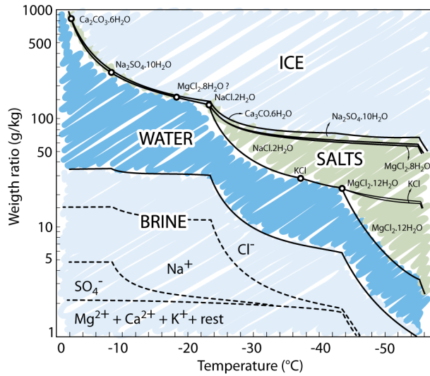
FIG. 7: Phase diagram of sea ice. After 157 . Color online.
