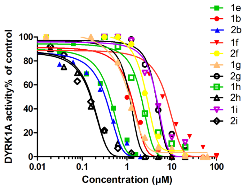
Figure 6: Dose-response of \Delta DYRK1A activity (normalized in the absence of inhibitor, expressed as percentage) obtained with varied concentration of 3-phenyl-7-azaindole derivatives 1e,b,f-i and 2b,f-i (0.02 – 100 \mu M) with 50 \mu M of ATP.
