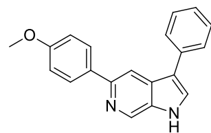
1a IC_{50} = 17.0 \mu M
