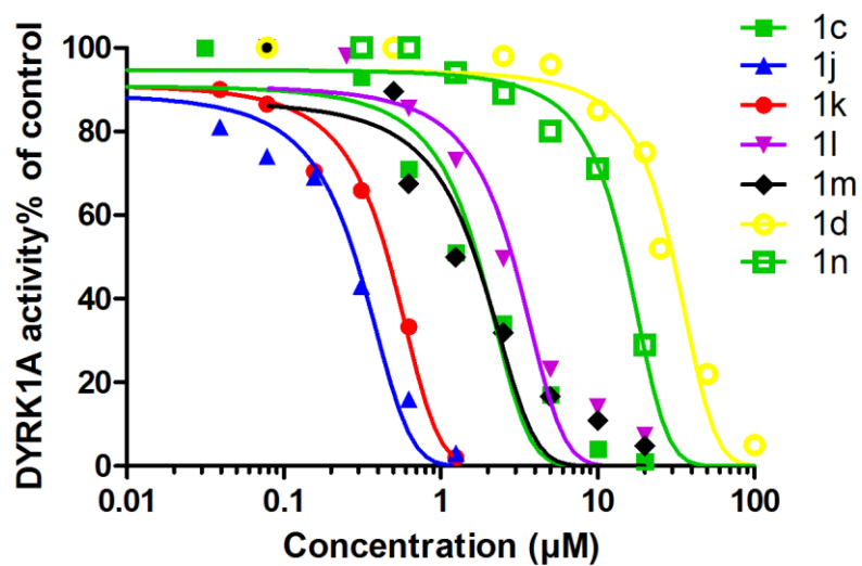
Figure 7: Dose-response of \Delta DYRK1A activity (normalized in the absence of inhibitor, expressed as percentage) obtained with varied concentration of polmethoxy 3,5-diaryl-7-azaindole derivatives 1c,d,j-n (0.02 – 100 \mu M) with 50 \mu M of ATP.
