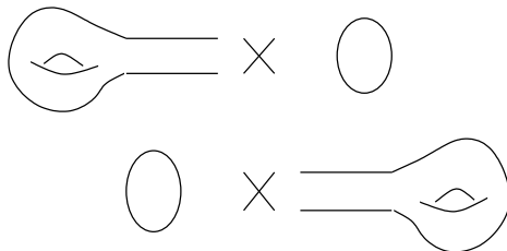
Figure 1: Manifold containing a thickened torus
