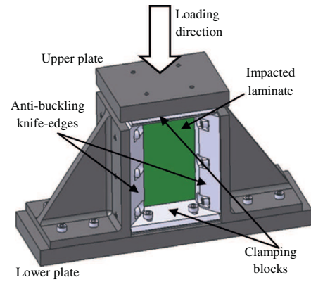
Fig. 3. CAI setup.
