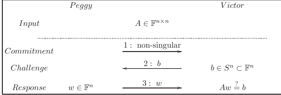
Figure 2: Blackbox interactive certificate of non-singularity
