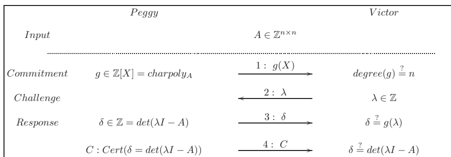
Figure 1: Interactive certificate for the characteristic polynomial
