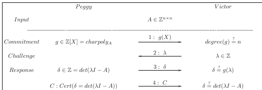
Figure 1: Interactive certificate for the characteristic polynomial
