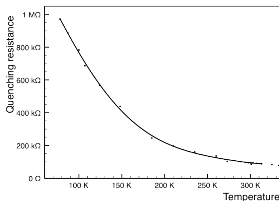
Figure 5. Quenching resistance R_Q as a function of the temperature. R_Q is extract from the figure 4 and by multiplying R_Q/N by the number of SiPM cells ( N=100 ).
