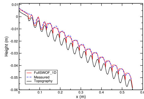
(b) Measured topography, experimental water surface and water surface computed by FullSWOF_1D (Simulation with 1104 cells at T = 10 \text{ s} ).
