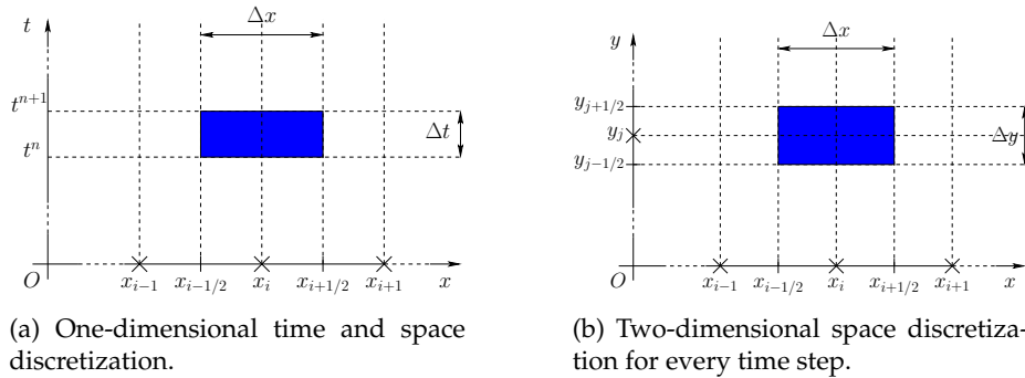
Figure 3: Discretization of time and space in FullSWOF.
