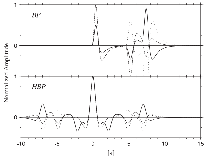
Figure 1. Time profiles of the stacked Green's function (top) and the stacked autocorrelation function of the Green's function (bottom) for a strike-slip point source on a vertical fault (solid lines). Those profiles for dip-slip point sources on a vertical fault (dotted lines) and on a thrust fault with a dip angle of 30^\circ (broken lines) are also shown. All point sources are put at a depth of 15 km. Observation stations are distributed every 10^\circ with the radial distance from 30^\circ to 90^\circ and all azimuthal direction. These time profiles represent the left-hand side of eq. (8) for top and that of eq. (17) for bottom. In order to obtain a sharp image by the BP and HBP analyses, these profiles must be close to the delta function. When an impulse slip was given at the point source, these profiles correspond to the time-evolving image of BP (top) and HBP (bottom) at the location of the point source.
