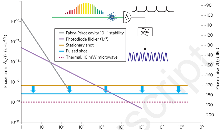
Figure 1 | Power spectral density of random phase for a 10-GHz femtosecond frequency comb detected with a high-power photodiode and expressed in terms of different units. The brown and light-blue lines are the shot noise given by Quinlan et al. 1 in the stationary and pulsed shot-noise regimes, respectively. By further reducing the shot noise, the pulsed shot-noise floor could reach the thermal noise (dashed line), unless the microwave power increases proportionally. Flicker ( 1/f ) noise is inherent in the detectors; the lowest flicker noise is observed at -133 dBc at 1 Hz (solid purple line). Owing to the photodiode flicker, the full advantages of the pulsed-shot regime are attained only at 100 kHz and beyond. At the lowest frequencies, the flicker-of-frequency noise of the Fabry-Pérot cavity (grey line with slope 1/f^2 ) may limit the spectral purity.
