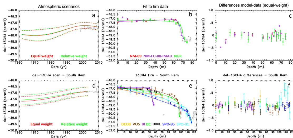
Fig. 5. Multi-site \delta^{13}\text{C}(\text{CH}_4) trend reconstructions ( a and d ), the model fit of the firn data ( b and e ) and the difference between model and data ( c and f ). NH sites ( a , b and c ) and SH sites ( d , e and f ). Two multi-site inversions are shown in ( a ) and ( d ), one giving equal weight to each site (red lines) and one weighting each site by the RMS difference of the single site reconstruction (Fig. 2) to the data (green lines). The light grey line (left panel) represents air-archive results from Cape Grim (Francey et al., 1998) and continuous atmospheric monitoring data from the NOAA-ESRL network.
