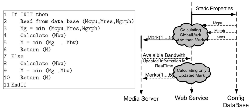
Figure 14: WAVA Algorithm
