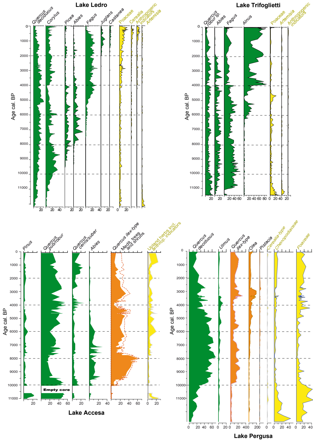
Fig. 2. Simplified pollen diagrams for the following: Lake Ledro deep core “LL081” (Joannin et al., 2013), Lake Accesa littoral core “AC3/4” (Drescher-Schneider et al., 2007), Lake Trifoglietti (Joannin et al., 2012) and Lake Pergusa (Sadori and Narcisi, 2001). The chronology of the four pollen records is based on radiocarbon dates compiled in Table 1. More details on each chronology are given in the references papers.
