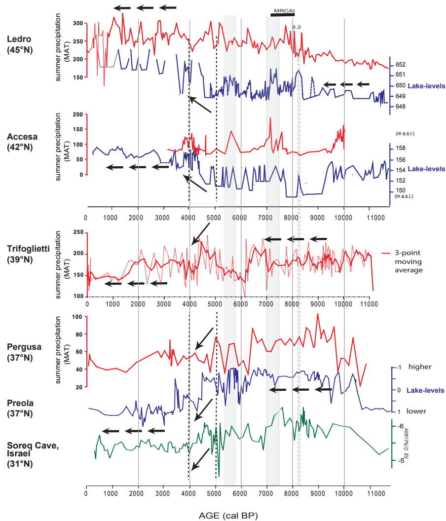
Fig. 6. Comparison between pollen-inferred summer precipitation (MAT only) and lake-level variations at Lakes Ledro, Accesa, Trifoglietti and Pergusa. More details on the lake-level data are given in Magny et al. (2012a) for Lake Ledro, Magny et al. (2007) for Lake Accesa, and Magny et al. (2011) for Lake Preola (Sicily). Oxygen isotope data based on speleothem from Soreq Cave, Israel, is also plotted for comparison with eastern Mediterranean sites (Bar-Matthews and Ayalon, 2011; Bar-Matthews et al., 1998; Vaks et al., 2006). MRCAI = period of maximal rate of change in annual insolation.
