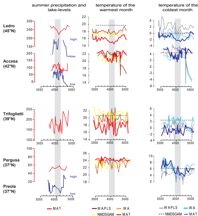
Fig. 8. Synthesis figure for the 4.2 kyr event in Italy, and comparison with lake-level data.
