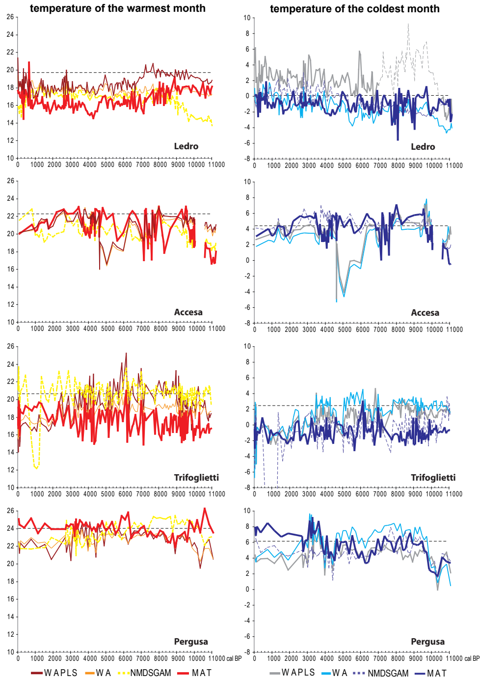
Fig. 3. Pollen-based temperatures (warmest and coldest month). Climate values are estimated using four methods: the modern analogue technique (MAT), the non-metric multidimensional scaling/generalized additive model method (NMDS/GAM), weighted averaging (WA), and weighted-average partial least-squares regression (WAPLS).
