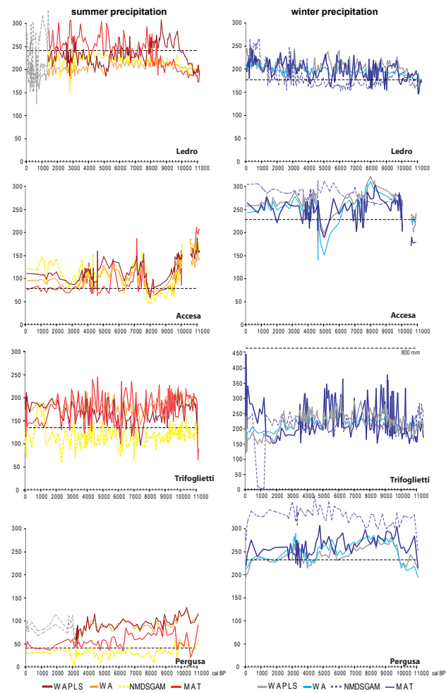
Fig. 4. Pollen-based seasonal precipitation (winter = sum of December, January, February precipitation, and summer = sum of June, July, August precipitation, in mm) values for the four lakes estimated with the methods listed in Fig. 3. Modern values are indicated with a horizontal grey dotted line. The thin dotted grey curve (summer precipitation, Ledro and Pergusa) corresponds to unrealistic values.
