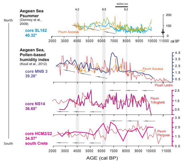
Fig. 7. Contrasting precipitation patterns in Italy and in Aegean Sea during the Holocene. Psum = Psummer (MAT only) as in Fig. 4, from each lake pollen record (dotted orange: Accessa; red: Ledro, Trifoglietti and Pergusa; units same as Fig. 6).
