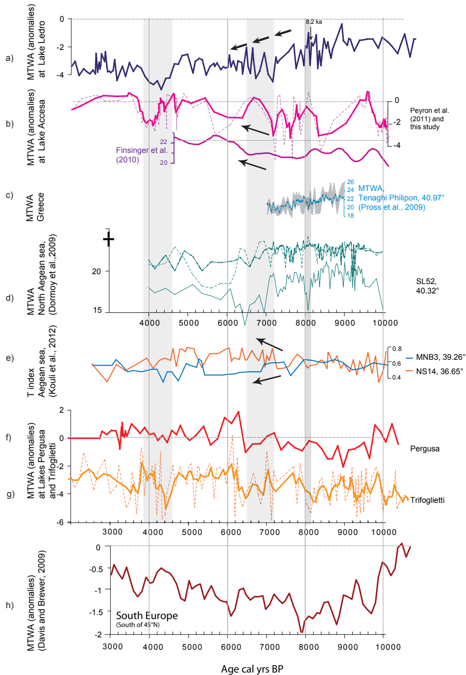
Fig. 5. Synthesis figure for selected Mediterranean temperature records. (a) Pollen-inferred temperature of the warmest month for Lake Ledro (as for Fig. 3), MAT only. (b) Pollen-inferred temperature of the warmest month for (1, pink curve) Lake Accessa littoral core, MAT only (as for Fig. 3), and (2, purple curve) Lake Accessa profundal core, WAPLS only (Finsinger et al., 2010). (c) Pollen-inferred temperature of the warmest month for Tenaghi Philippon, Greece, MAT only (Pross et al., 2009). (d) Pollen-inferred temperature of the warmest month for the marine core SL152, Aegean Sea, (Dormoy et al., 2009) with three methods (short dotted line: MAT; blue line: PLS; long dotted line: NMDS/GAM). (e) Pollen-based temperature index “T index” for the marine cores MNB3 (North Aegean Sea), and NS14 (South Aegean Sea), (Kouli et al., 2012). (f) Pollen-inferred temperature of the warmest month for Lake Pergusa (as for Fig. 3), MAT only. (g) Pollen-inferred temperature of the warmest month for Lake Trifoglietti (as for Fig. 3), MAT only; the curve of temperature is calculated with a moving average (bold curve) and raw values are also plotted (dotted curve). (h) Reconstruction of temperatures of the warmest month (anomalies) for Southern Europe based on pollen data from over 500 pollen sites from across Europe, MAT only (Davis and Brewer, 2009; Davis et al., 2003).
