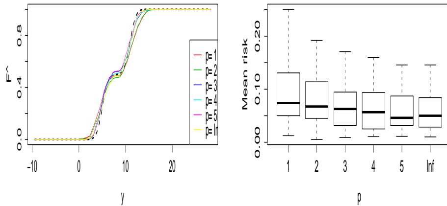
FIGURE 4. First column: Plots of true conditional c.d.f. (black dotted line) versus estimators \widehat{F}_{h^*,p}^{x_0} , for p \in \{1, 2, 3, 4, 5, \infty\} , calculated from a sample of size n = 500 (thin lines), with x_0 a copy of X , in Example 1 (first line) and 2 (second line) with process (a). Second column: Boxplots of the risks of 50 previous estimators for the same values of p .
