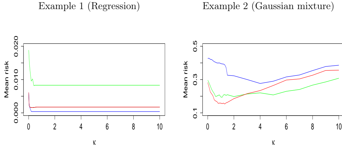
FIGURE 2. Plot of approximated mean risk with respect to \kappa . Blue curves: Process (a) - H_{X,L} . Green curves: Process (b) - H_{X,M} . Red curves: Process (c) - H_{X,F} .
