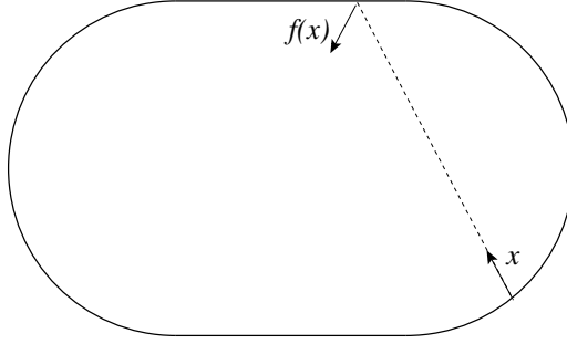
FIGURE 3. The billiard map f .
