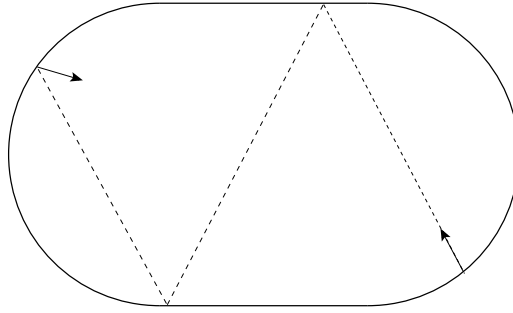
FIGURE 2. The stadium billiard
