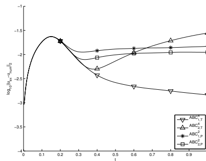
Fig. 9. Comparison of the error norm \log_{10} (\|u_{ex}(\cdot, t) - u_{num}(\cdot, t)\|_{L^2(\Omega_2)}) for different ABCs.
