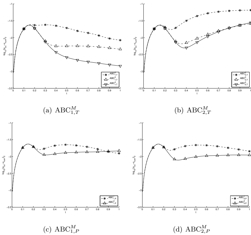
Fig. 8. Evolution of the error norm \log_{10} (\|u_{ex}(\cdot, t) - u_{num}(\cdot, t)\|_{L^2(\Omega_2)}) with respect to the ABC order.
