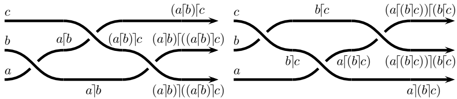
FIGURE 7. Colouring braids using the rule (1.24) is invariant under braid relations if and only if the birack laws (1.21)–(1.23) are obeyed.
