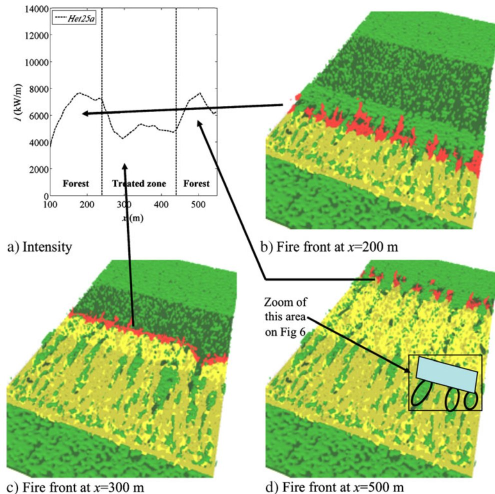
Fig. 5 a Fire intensity variation along the forest-treated zone–forest pattern (case het25 : C=25\% , L=4 m). Fire behavior at three locations: within the upwind forest ( b ), within the treated zone ( c ), and within the downwind forest ( d )
