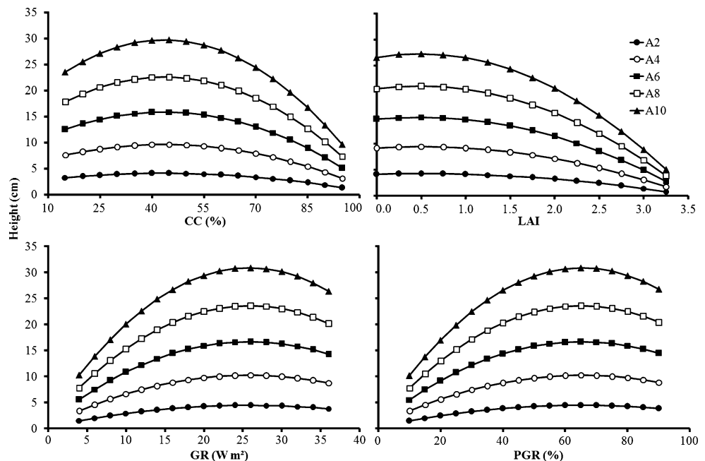
Fig. 1 Model prediction of average seedling height after harvesting according to their age (A2 to A10 years) and crown cover (CC) (%), effective leaf area index (LAI), global radiation (GR) (W m 2 ) and percentage of global radiation (PGR) (%) at understory level transmitted through the canopy in Nothofagus pumilio forests
