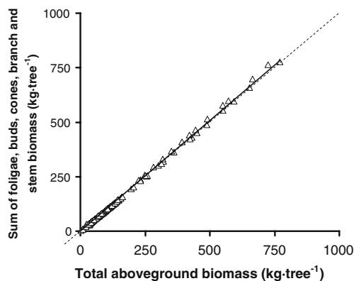
Fig. 3 Plot of the sum of predicted values of the biomass components versus total aboveground biomass estimates (1:1 line/broken line; linear regression bold line ). Values are produced by the models retained and corresponding values are given in bold font in Table 1
