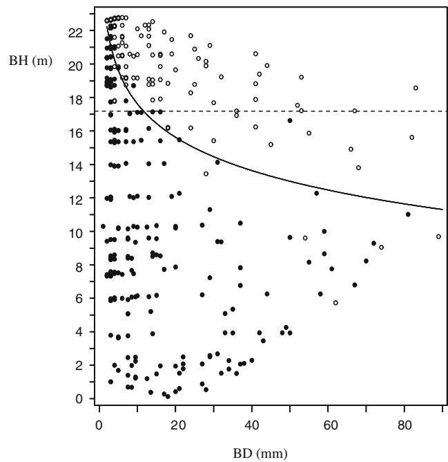
Fig. 5 Plot of branch diameter vs. insert height in a sample tree (R12 3). Dot: dead branch. Circle: living branch. The solid line shows the isoproability for a branch to be dead or alive according to the model (Eq. 10). The horizontal dashed line represents the height of the lowest live whorl (HLW)
